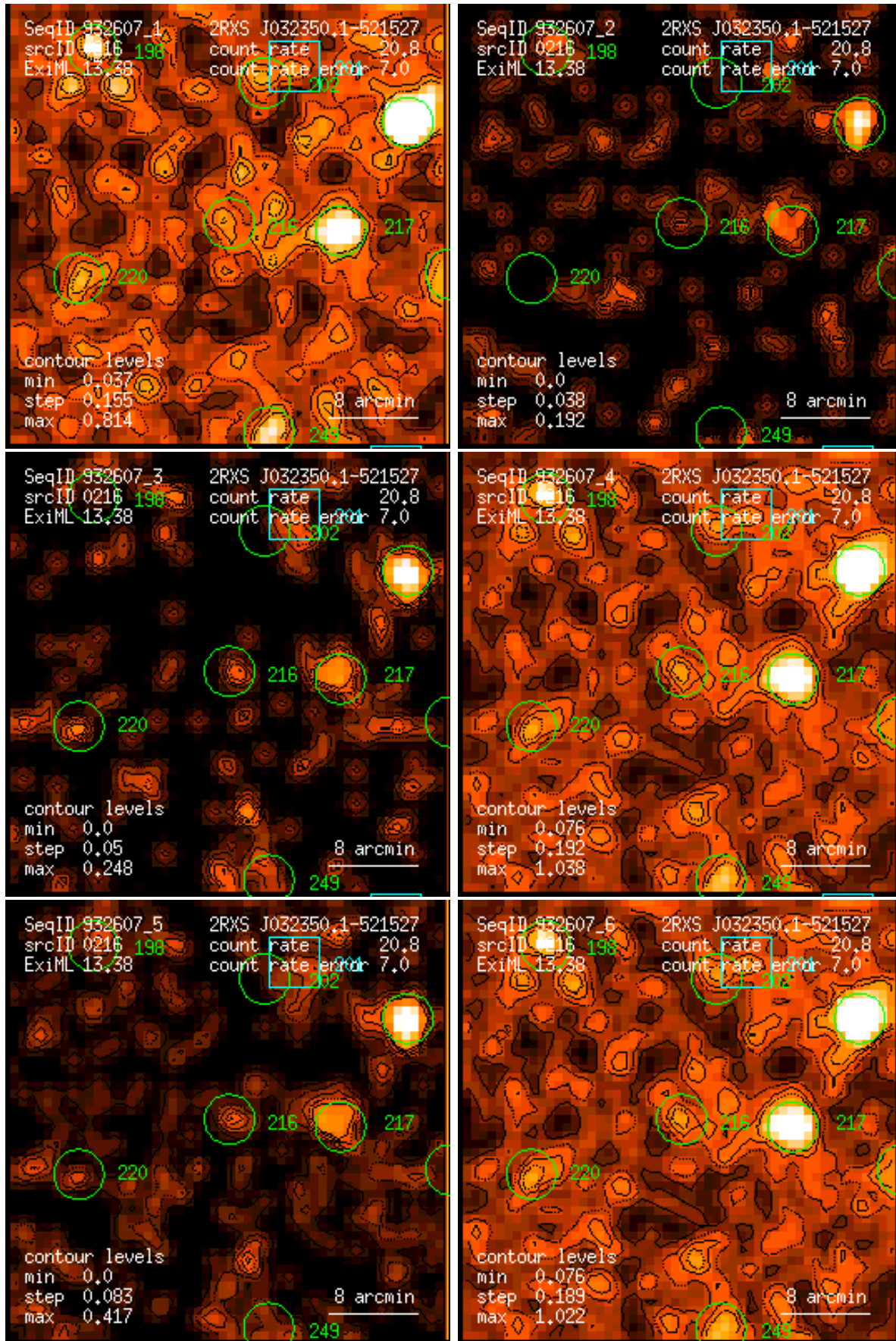
Figure 216: RASS 932607: detection 0216: band rate images, Gaussian filter: (1) PSPC channels 11 – 41, (2) 52 – 90, (3) 91 – 201, (4) 11 – 235, (5) 52 – 201, (6) 11 – 201. Broad band rates in counts/ks. Band rate contour levels in counts/ks/arcmin 2 .
