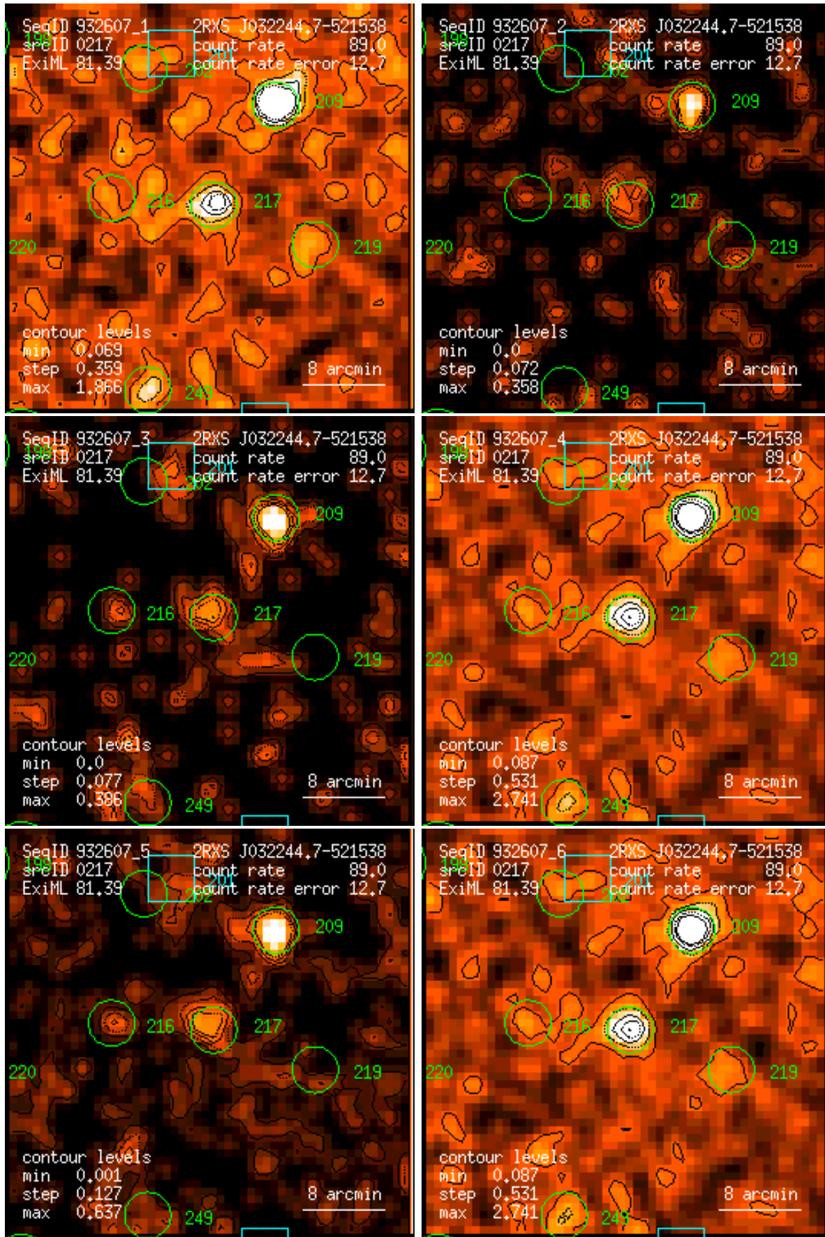
Figure 217: RASS 932607: detection 0217: band rate images, Gaussian filter: (1) PSPC channels 11 – 41, (2) 52 – 90, (3) 91 – 201, (4) 11 – 235, (5) 52 – 201, (6) 11 – 201. Broad band rates in counts/ks. Band rate contour levels in counts/ks/arcmin 2 .
