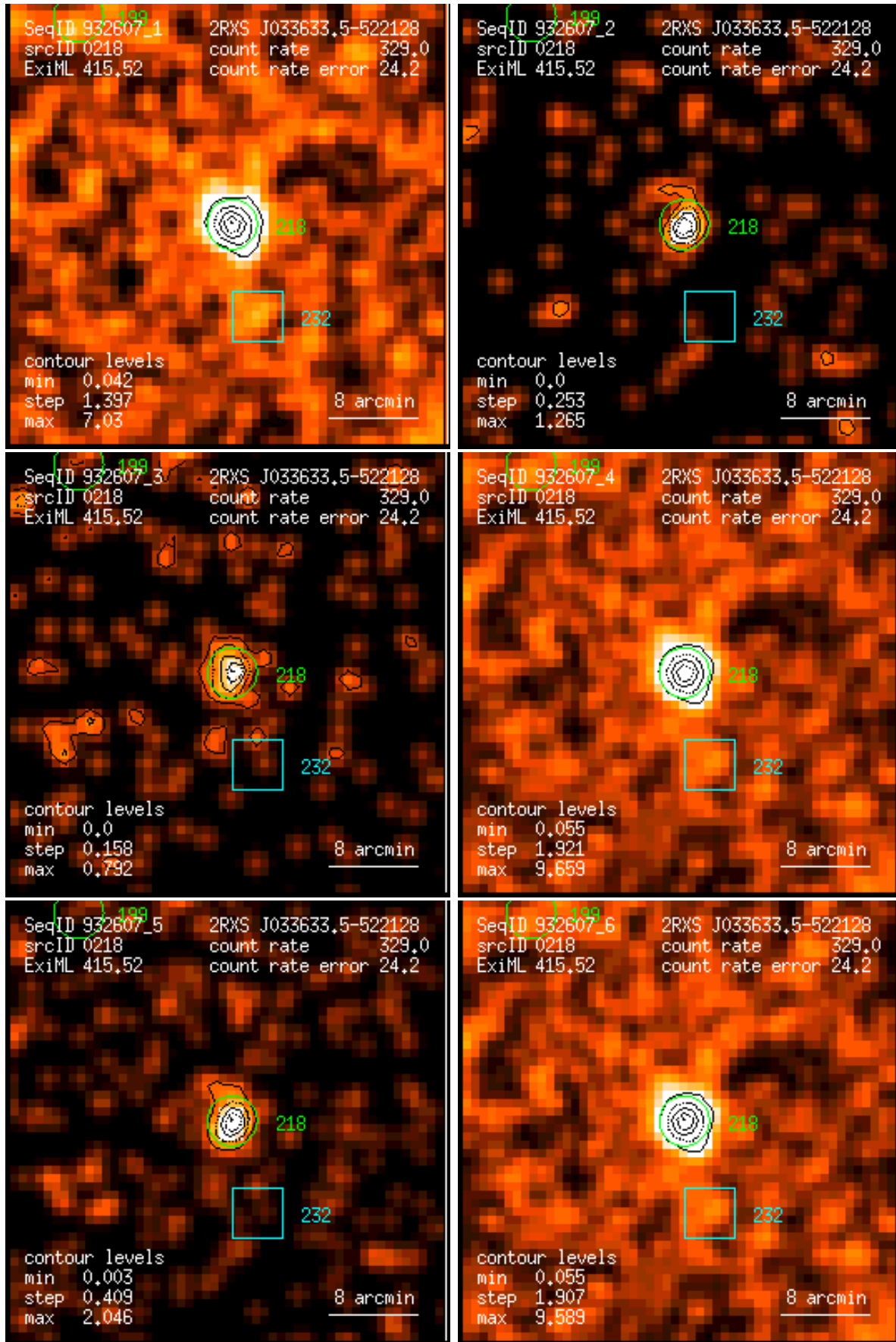
Figure 218: RASS 932607: detection 0218: band rate images, Gaussian filter: (1) PSPC channels 11 – 41, (2) 52 – 90, (3) 91 – 201, (4) 11 – 235, (5) 52 – 201, (6) 11 – 201. Broad band rates in counts/ks. Band rate contour levels in counts/ks/arcmin 2 .
