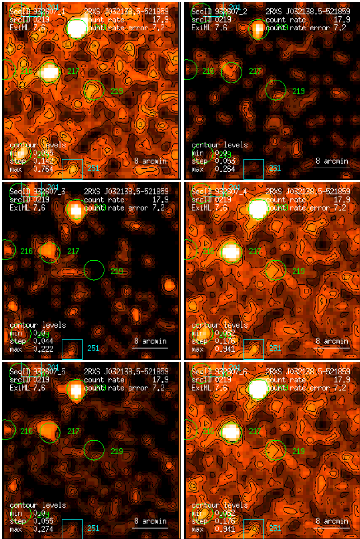
Figure 219: RASS 932607: detection 0219: band rate images, Gaussian filter: (1) PSPC channels 11 – 41, (2) 52 – 90, (3) 91 – 201, (4) 11 – 235, (5) 52 – 201, (6) 11 – 201. Broad band rates in counts/ks. Band rate contour levels in counts/ks/arcmin 2 .
