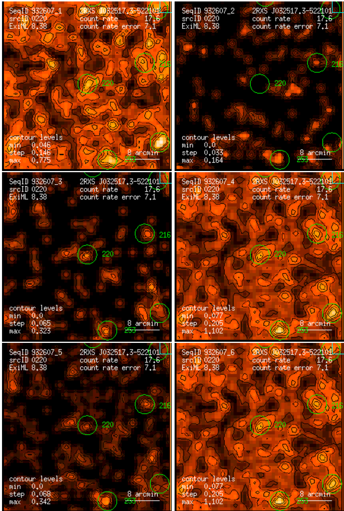
Figure 220: RASS 932607: detection 0220: band rate images, Gaussian filter: (1) PSPC channels 11 – 41, (2) 52 – 90, (3) 91 – 201, (4) 11 – 235, (5) 52 – 201, (6) 11 – 201. Broad band rates in counts/ks. Band rate contour levels in counts/ks/arcmin 2 .
