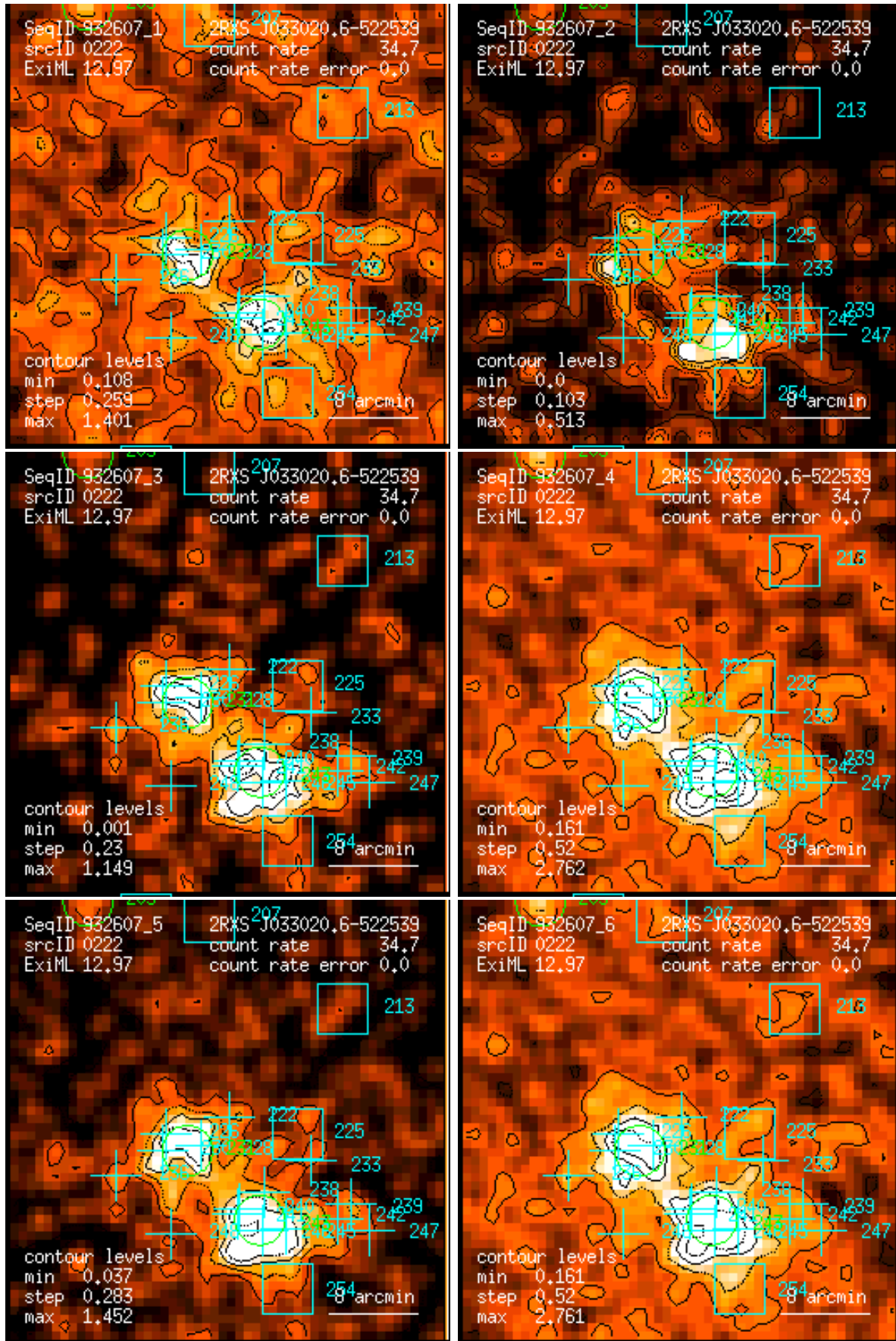
Figure 222: RASS 932607: detection 0222: band rate images, Gaussian filter: (1) PSPC channels 11 – 41, (2) 52 – 90, (3) 91 – 201, (4) 11 – 235, (5) 52 – 201, (6) 11 – 201. Broad band rates in counts/ks. Band rate contour levels in counts/ks/arcmin 2 .
