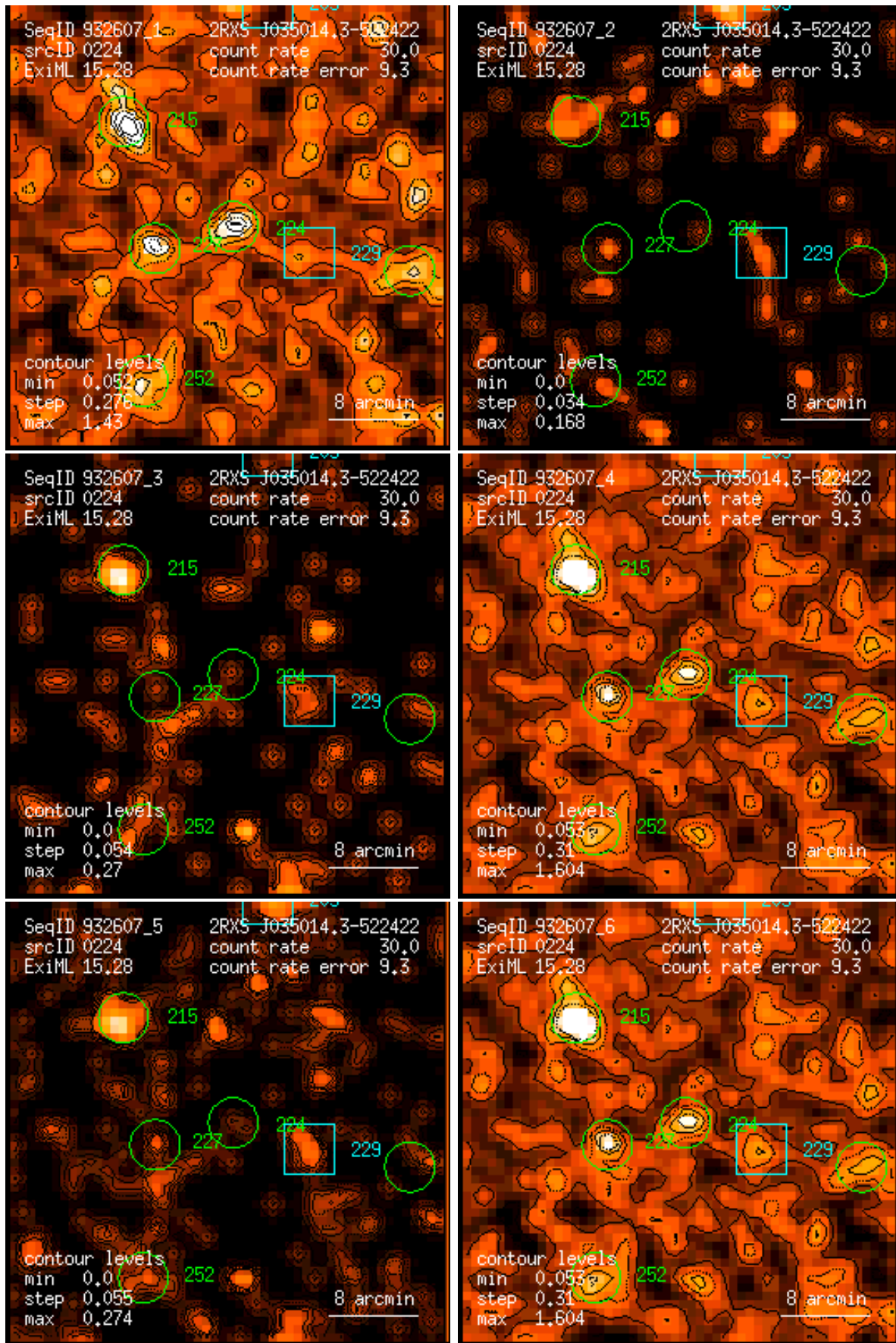
Figure 224: RASS 932607: detection 0224: band rate images, Gaussian filter: (1) PSPC channels 11 – 41, (2) 52 – 90, (3) 91 – 201, (4) 11 – 235, (5) 52 – 201, (6) 11 – 201. Broad band rates in counts/ks. Band rate contour levels in counts/ks/arcmin 2 .
