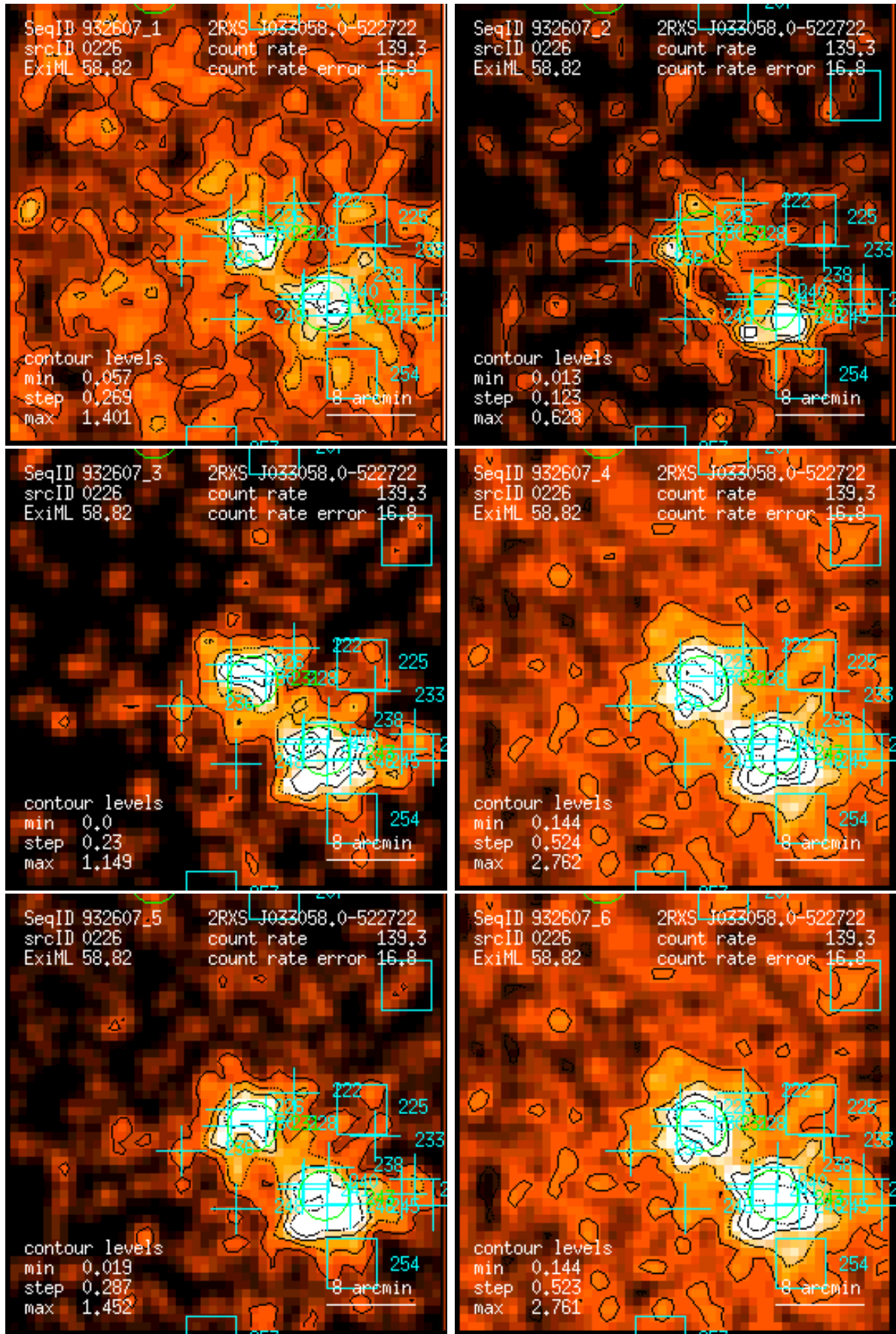
Figure 226: RASS 932607: detection 0226: band rate images, Gaussian filter: (1) PSPC channels 11 – 41, (2) 52 – 90, (3) 91 – 201, (4) 11 – 235, (5) 52 – 201, (6) 11 – 201. Broad band rates in counts/ks. Band rate contour levels in counts/ks/arcmin 2 .
