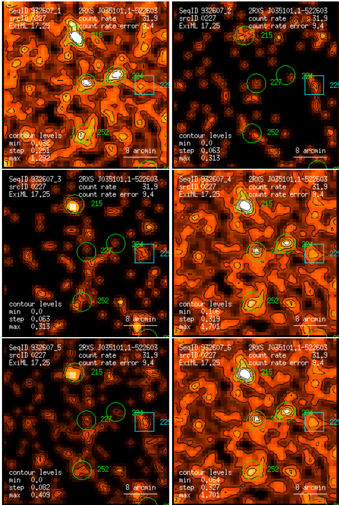
Figure 227: RASS 932607: detection 0227: band rate images, Gaussian filter: (1) PSPC channels 11 – 41, (2) 52 – 90, (3) 91 – 201, (4) 11 – 235, (5) 52 – 201, (6) 11 – 201. Broad band rates in counts/ks. Band rate contour levels in counts/ks/arcmin 2 .
