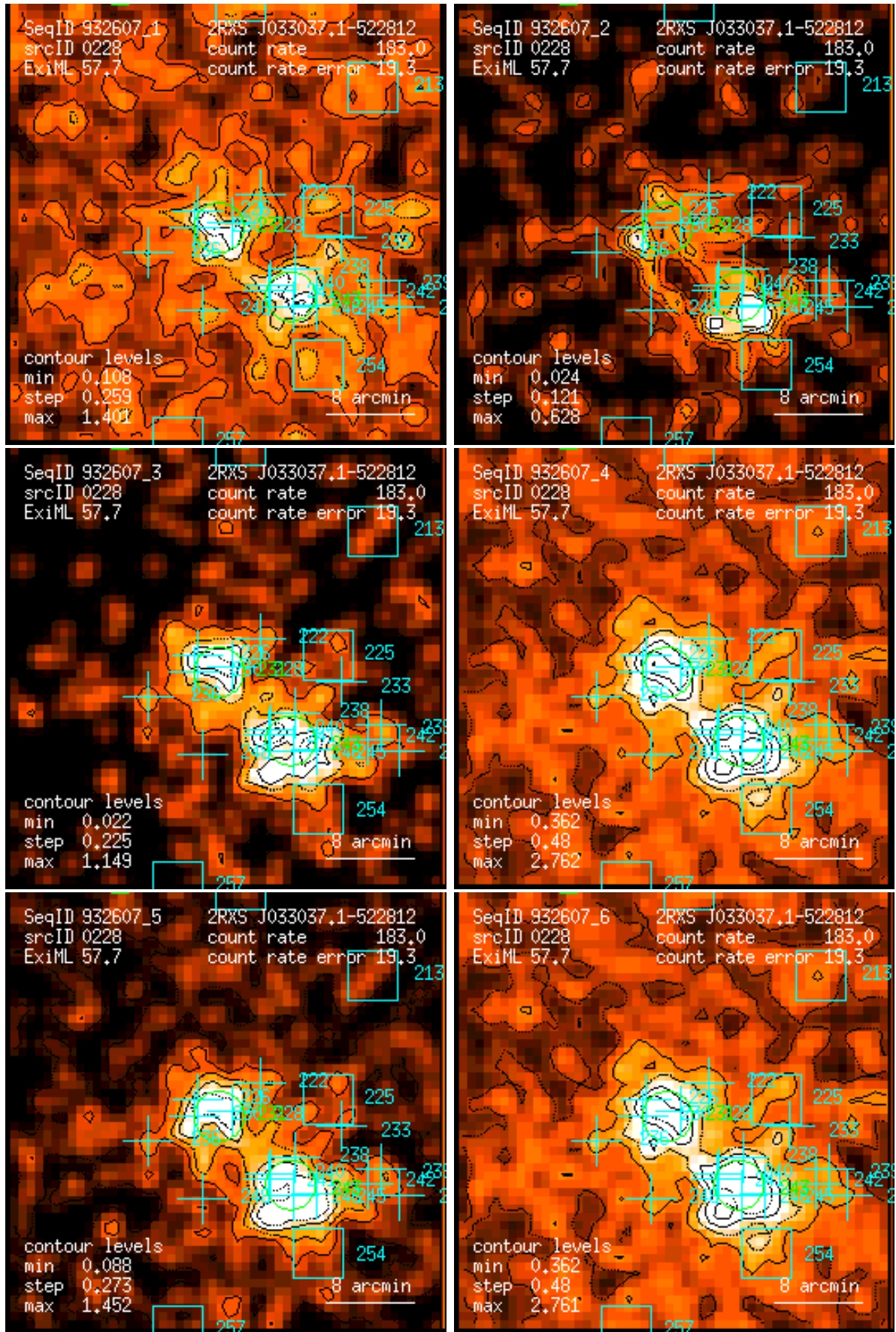
Figure 228: RASS 932607: detection 0228: band rate images, Gaussian filter: (1) PSPC channels 11 – 41, (2) 52 – 90, (3) 91 – 201, (4) 11 – 235, (5) 52 – 201, (6) 11 – 201. Broad band rates in counts/ks. Band rate contour levels in counts/ks/arcmin 2 .
