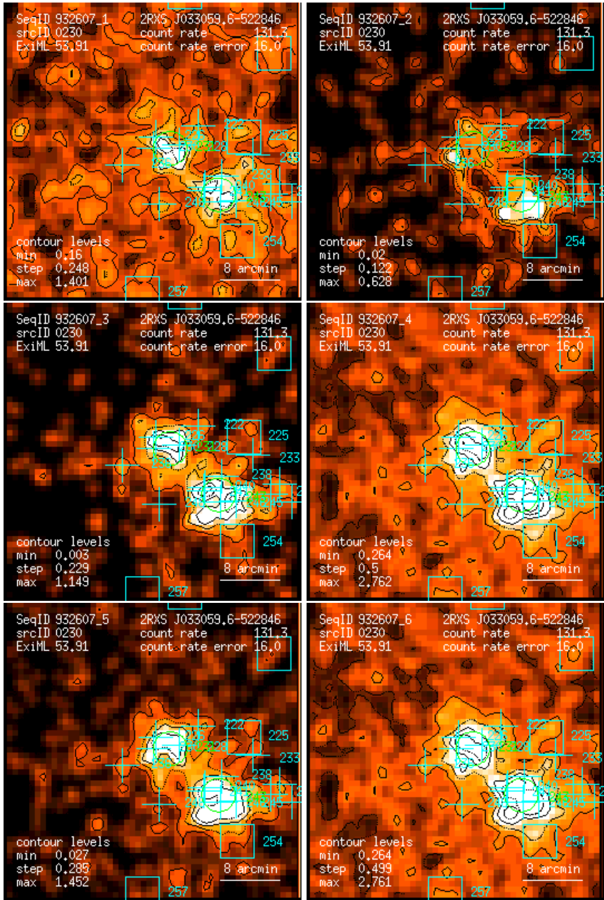
Figure 230: RASS 932607: detection 0230: band rate images, Gaussian filter: (1) PSPC channels 11 – 41, (2) 52 – 90, (3) 91 – 201, (4) 11 – 235, (5) 52 – 201, (6) 11 – 201. Broad band rates in counts/ks. Band rate contour levels in counts/ks/arcmin 2 .
