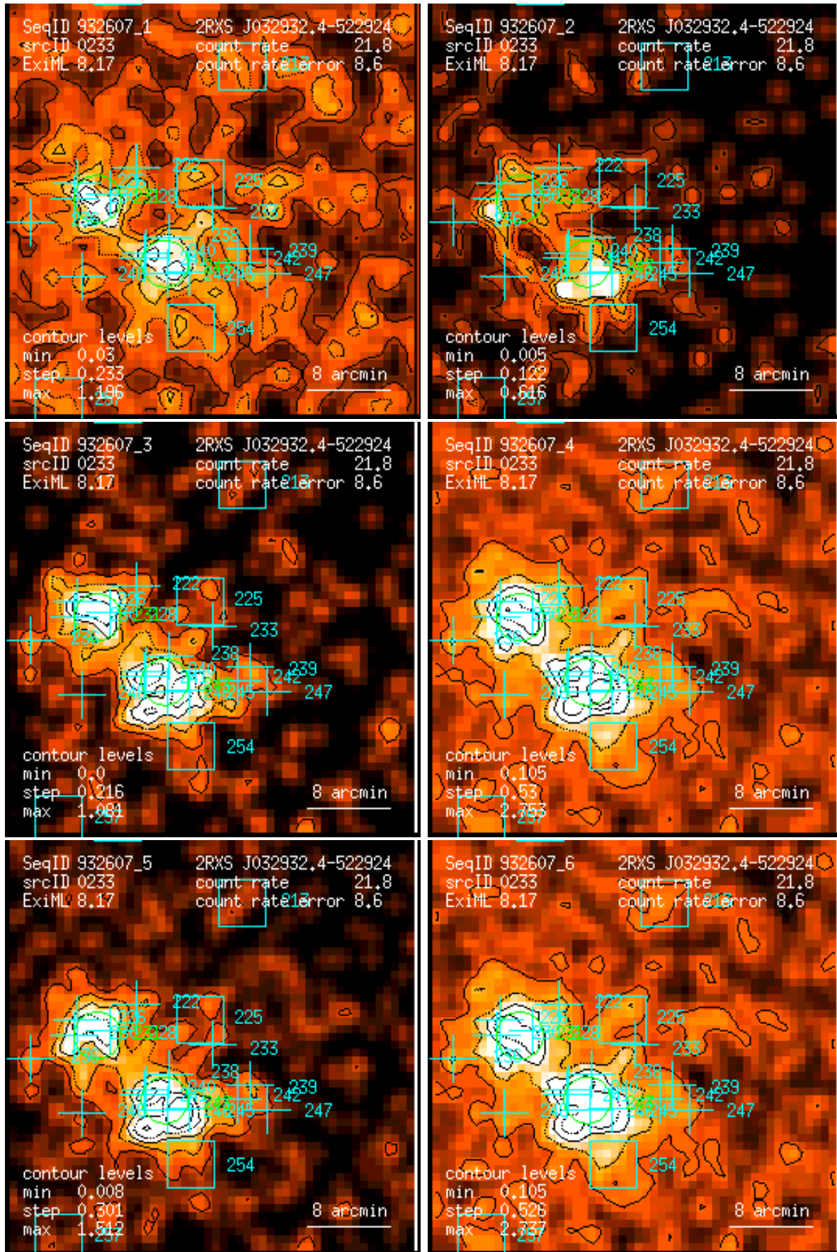
Figure 233: RASS 932607: detection 0233: band rate images, Gaussian filter: (1) PSPC channels 11 – 41, (2) 52 – 90, (3) 91 – 201, (4) 11 – 235, (5) 52 – 201, (6) 11 – 201. Broad band rates in counts/ks. Band rate contour levels in counts/ks/arcmin 2 .
