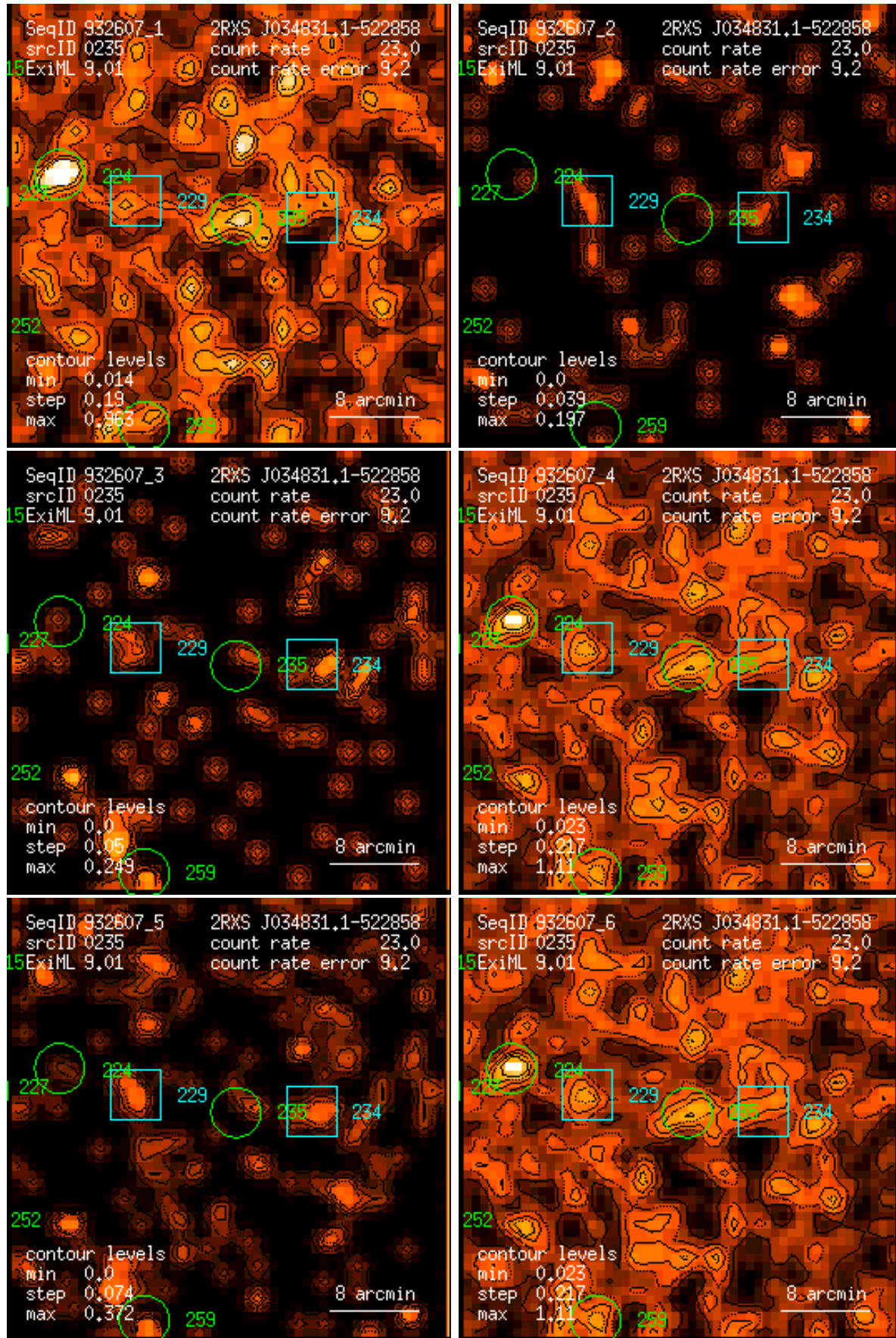
Figure 235: RASS 932607: detection 0235: band rate images, Gaussian filter: (1) PSPC channels 11 – 41, (2) 52 – 90, (3) 91 – 201, (4) 11 – 235, (5) 52 – 201, (6) 11 – 201. Broad band rates in counts/ks. Band rate contour levels in counts/ks/arcmin 2 .
