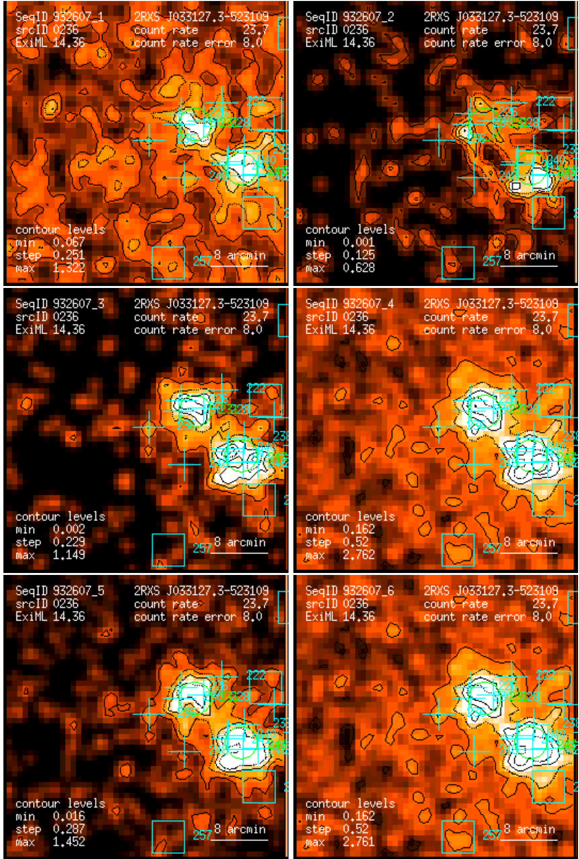
Figure 236: RASS 932607: detection 0236: band rate images, Gaussian filter: (1) PSPC channels 11 – 41, (2) 52 – 90, (3) 91 – 201, (4) 11 – 235, (5) 52 – 201, (6) 11 – 201. Broad band rates in counts/ks. Band rate contour levels in counts/ks/arcmin 2 .
