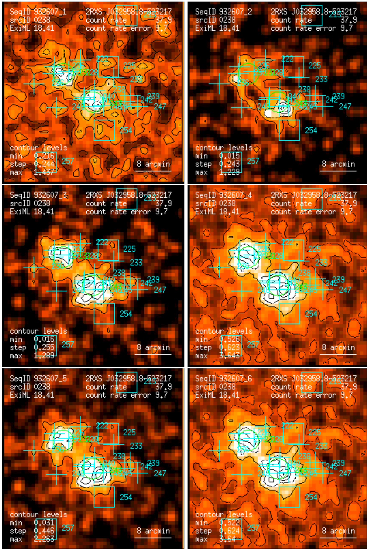
Figure 238: RASS 932607: detection 0238: band rate images, Gaussian filter: (1) PSPC channels 11 – 41, (2) 52 – 90, (3) 91 – 201, (4) 11 – 235, (5) 52 – 201, (6) 11 – 201. Broad band rates in counts/ks. Band rate contour levels in counts/ks/arcmin 2 .
