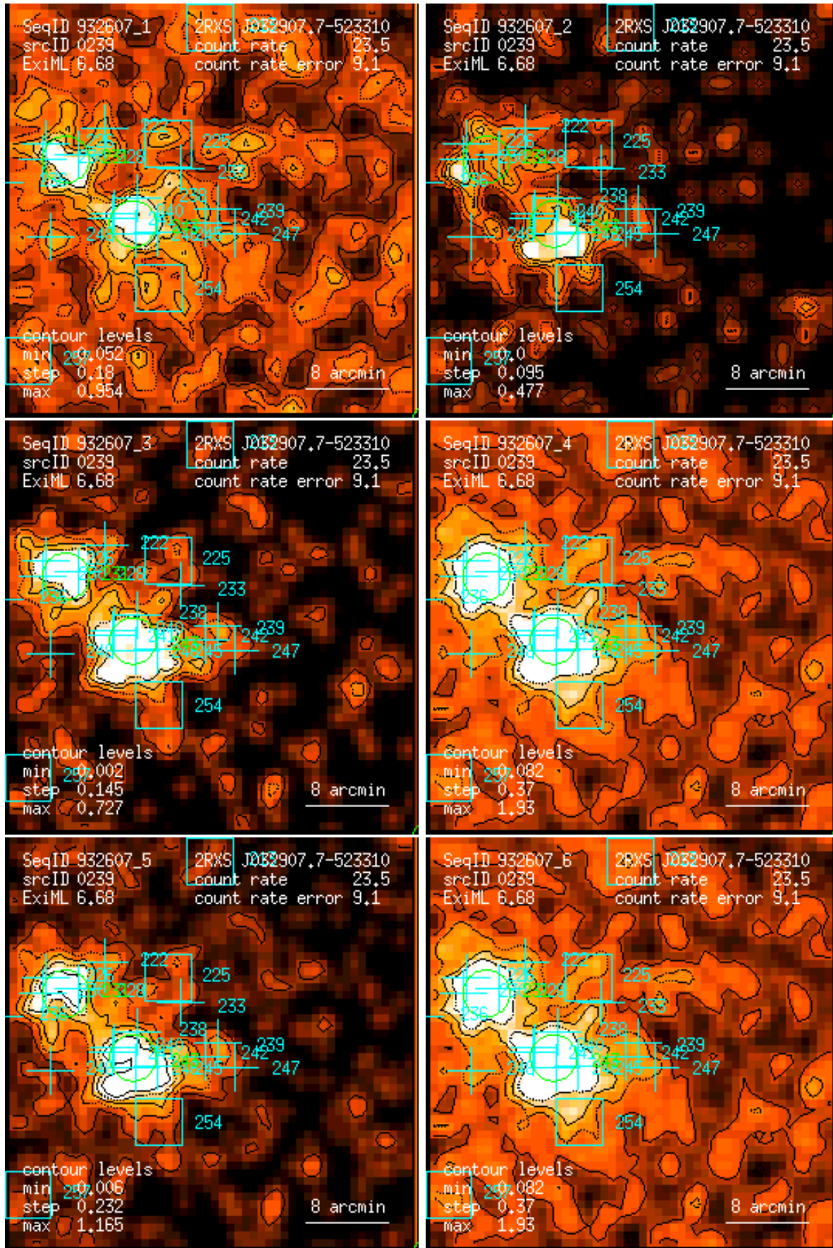
Figure 239: RASS 932607: detection 0239: band rate images, Gaussian filter: (1) PSPC channels 11 – 41, (2) 52 – 90, (3) 91 – 201, (4) 11 – 235, (5) 52 – 201, (6) 11 – 201. Broad band rates in counts/ks. Band rate contour levels in counts/ks/arcmin 2 .
