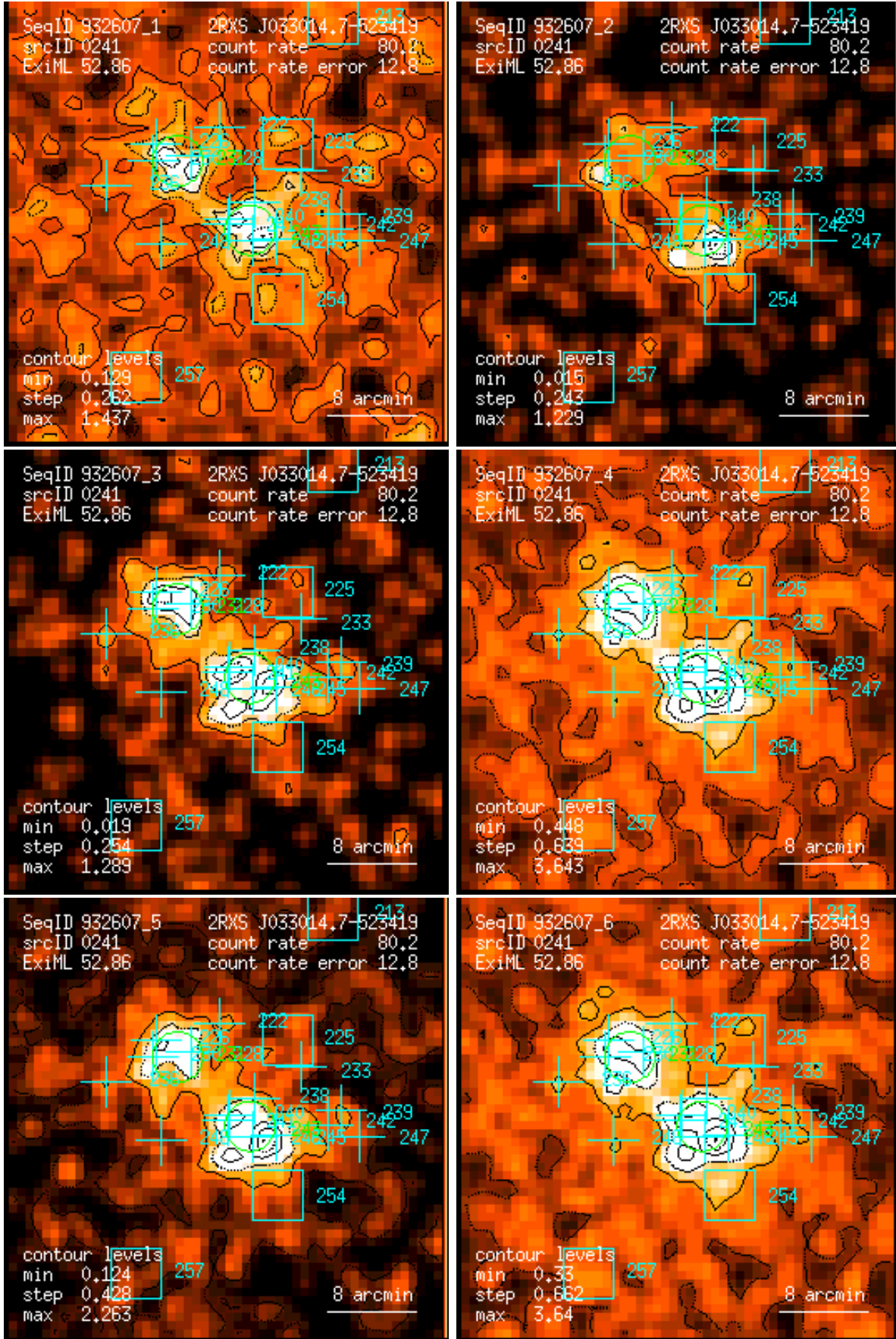
Figure 241: RASS 932607: detection 0241: band rate images, Gaussian filter: (1) PSPC channels 11 – 41, (2) 52 – 90, (3) 91 – 201, (4) 11 – 235, (5) 52 – 201, (6) 11 – 201. Broad band rates in counts/ks. Band rate contour levels in counts/ks/arcmin 2 .
