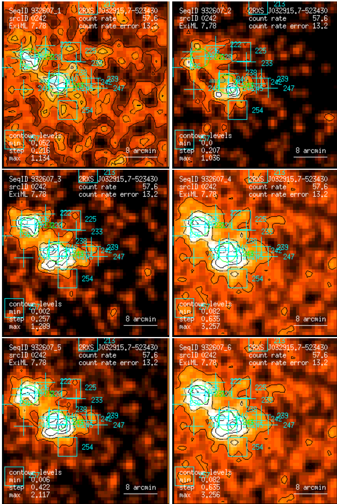
Figure 242: RASS 932607: detection 0242: band rate images, Gaussian filter: (1) PSPC channels 11 – 41, (2) 52 – 90, (3) 91 – 201, (4) 11 – 235, (5) 52 – 201, (6) 11 – 201. Broad band rates in counts/ks. Band rate contour levels in counts/ks/arcmin 2 .
