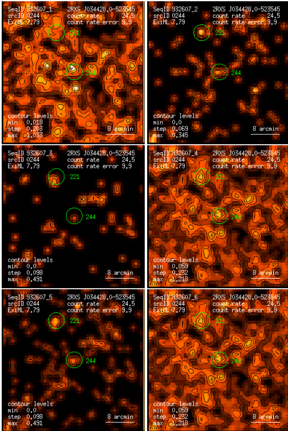
Figure 244: RASS 932607: detection 0244: band rate images, Gaussian filter: (1) PSPC channels 11 – 41, (2) 52 – 90, (3) 91 – 201, (4) 11 – 235, (5) 52 – 201, (6) 11 – 201. Broad band rates in counts/ks. Band rate contour levels in counts/ks/arcmin 2 .
