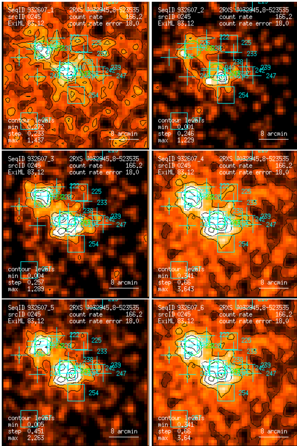
Figure 245: RASS 932607: detection 0245: band rate images, Gaussian filter: (1) PSPC channels 11 – 41, (2) 52 – 90, (3) 91 – 201, (4) 11 – 235, (5) 52 – 201, (6) 11 – 201. Broad band rates in counts/ks. Band rate contour levels in counts/ks/arcmin 2 .
