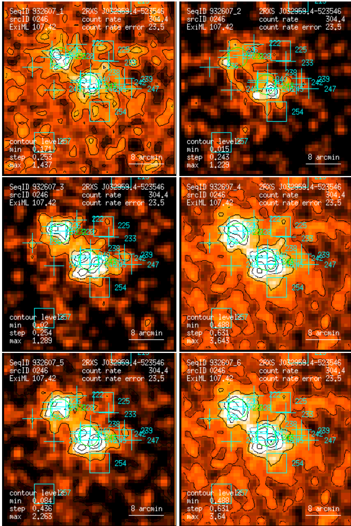
Figure 246: RASS 932607: detection 0246: band rate images, Gaussian filter: (1) PSPC channels 11 – 41, (2) 52 – 90, (3) 91 – 201, (4) 11 – 235, (5) 52 – 201, (6) 11 – 201. Broad band rates in counts/ks. Band rate contour levels in counts/ks/arcmin 2 .
