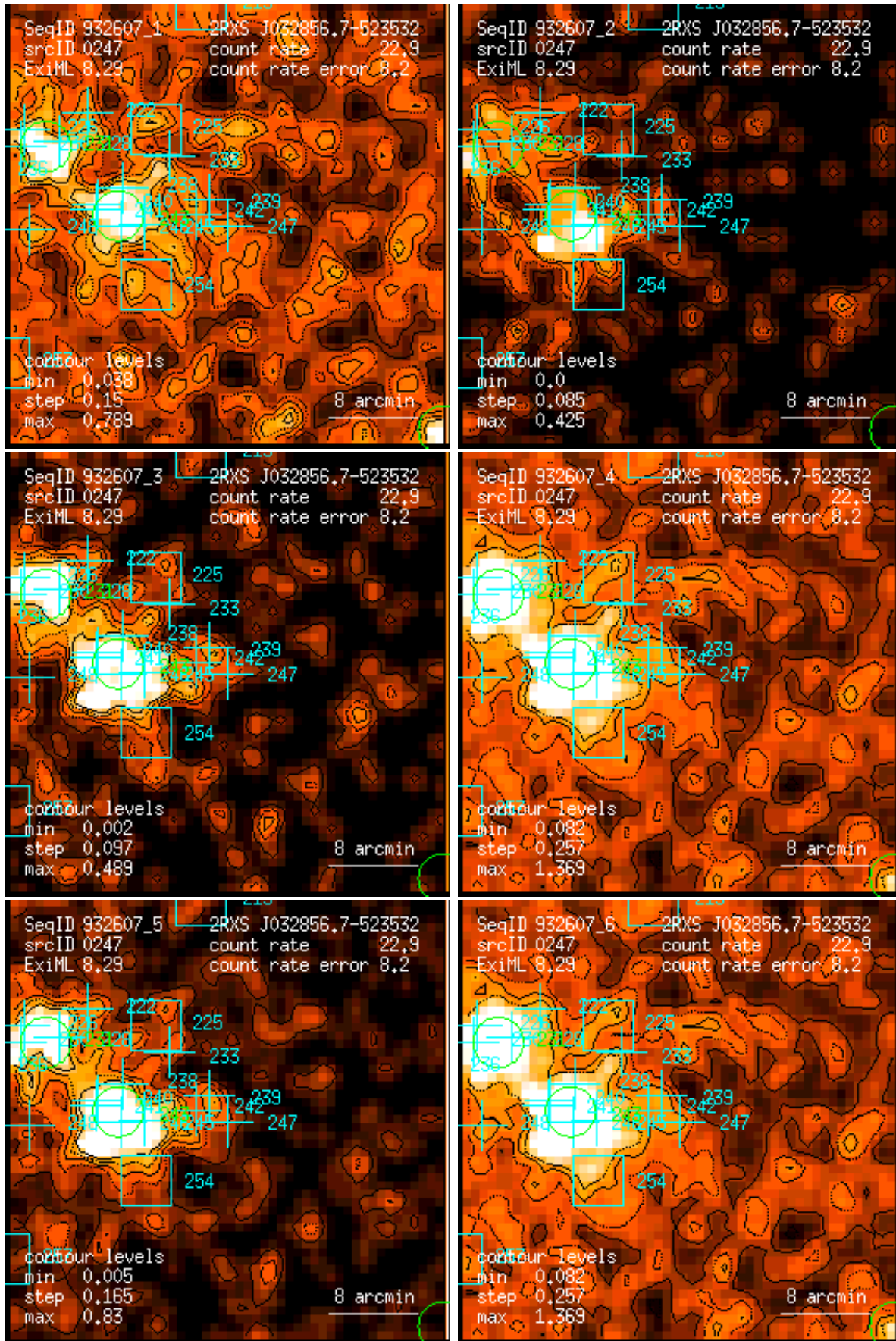
Figure 247: RASS 932607: detection 0247: band rate images, Gaussian filter: (1) PSPC channels 11 – 41, (2) 52 – 90, (3) 91 – 201, (4) 11 – 235, (5) 52 – 201, (6) 11 – 201. Broad band rates in counts/ks. Band rate contour levels in counts/ks/arcmin 2 .
