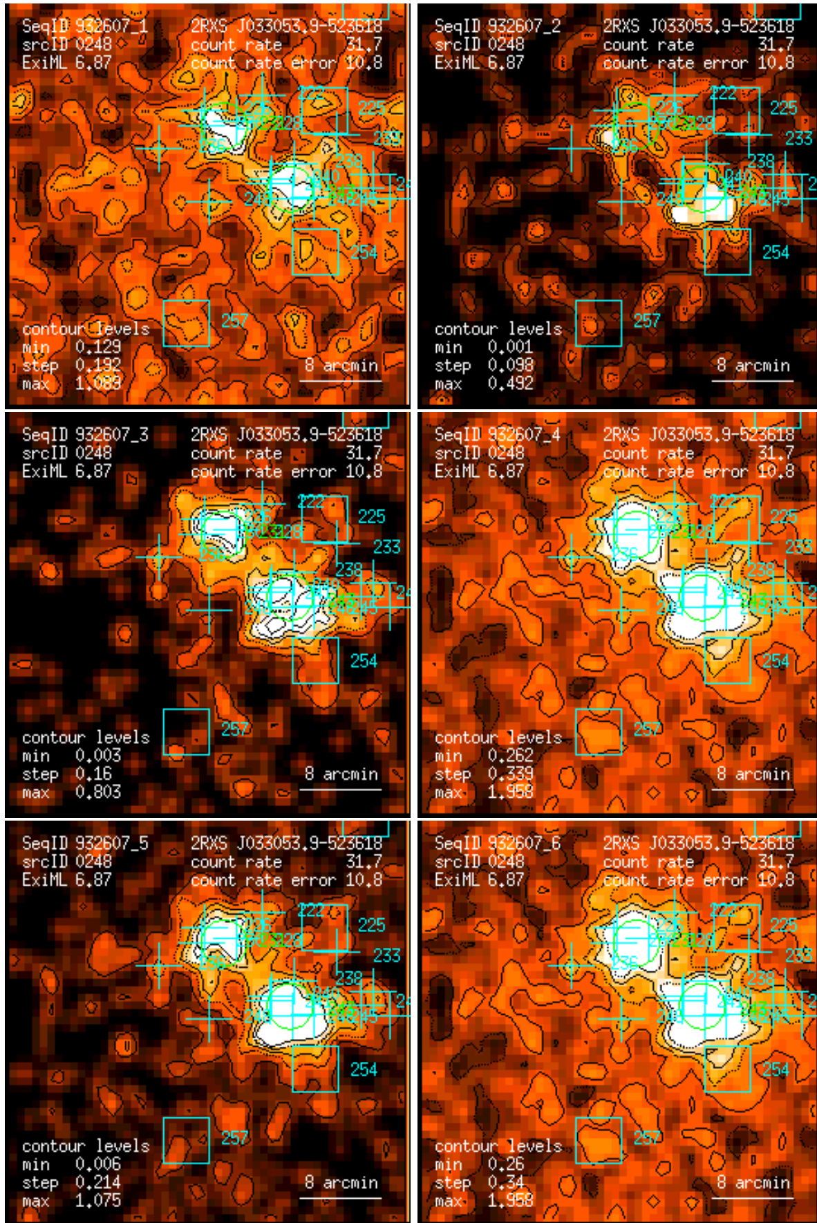
Figure 248: RASS 932607: detection 0248: band rate images, Gaussian filter: (1) PSPC channels 11 – 41, (2) 52 – 90, (3) 91 – 201, (4) 11 – 235, (5) 52 – 201, (6) 11 – 201. Broad band rates in counts/ks. Band rate contour levels in counts/ks/arcmin 2 .
