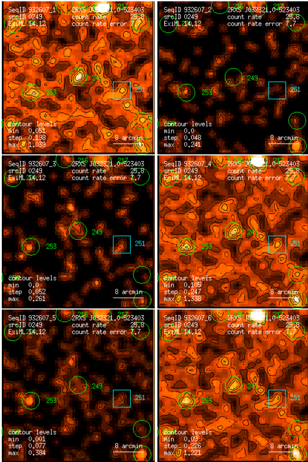
Figure 249: RASS 932607: detection 0249: band rate images, Gaussian filter: (1) PSPC channels 11 – 41, (2) 52 – 90, (3) 91 – 201, (4) 11 – 235, (5) 52 – 201, (6) 11 – 201. Broad band rates in counts/ks. Band rate contour levels in counts/ks/arcmin 2 .
