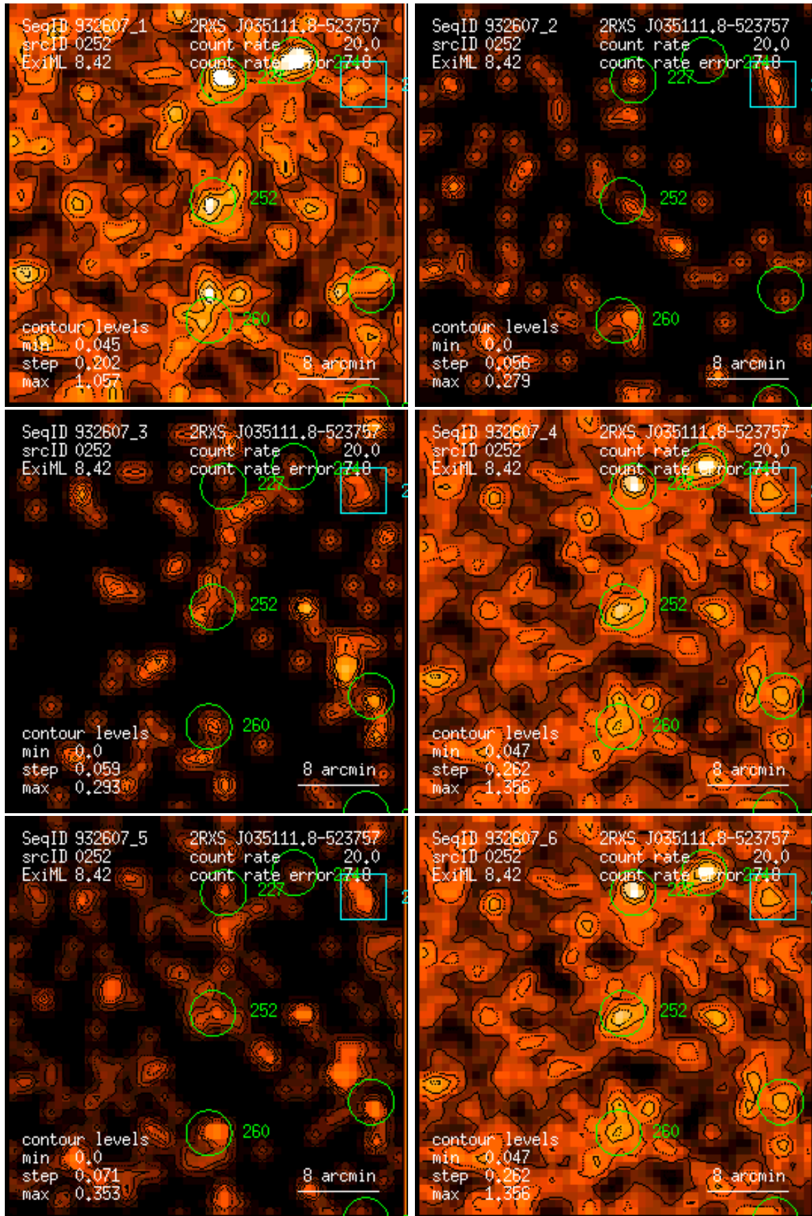
Figure 252: RASS 932607: detection 0252: band rate images, Gaussian filter: (1) PSPC channels 11 – 41, (2) 52 – 90, (3) 91 – 201, (4) 11 – 235, (5) 52 – 201, (6) 11 – 201. Broad band rates in counts/ks. Band rate contour levels in counts/ks/arcmin 2 .
