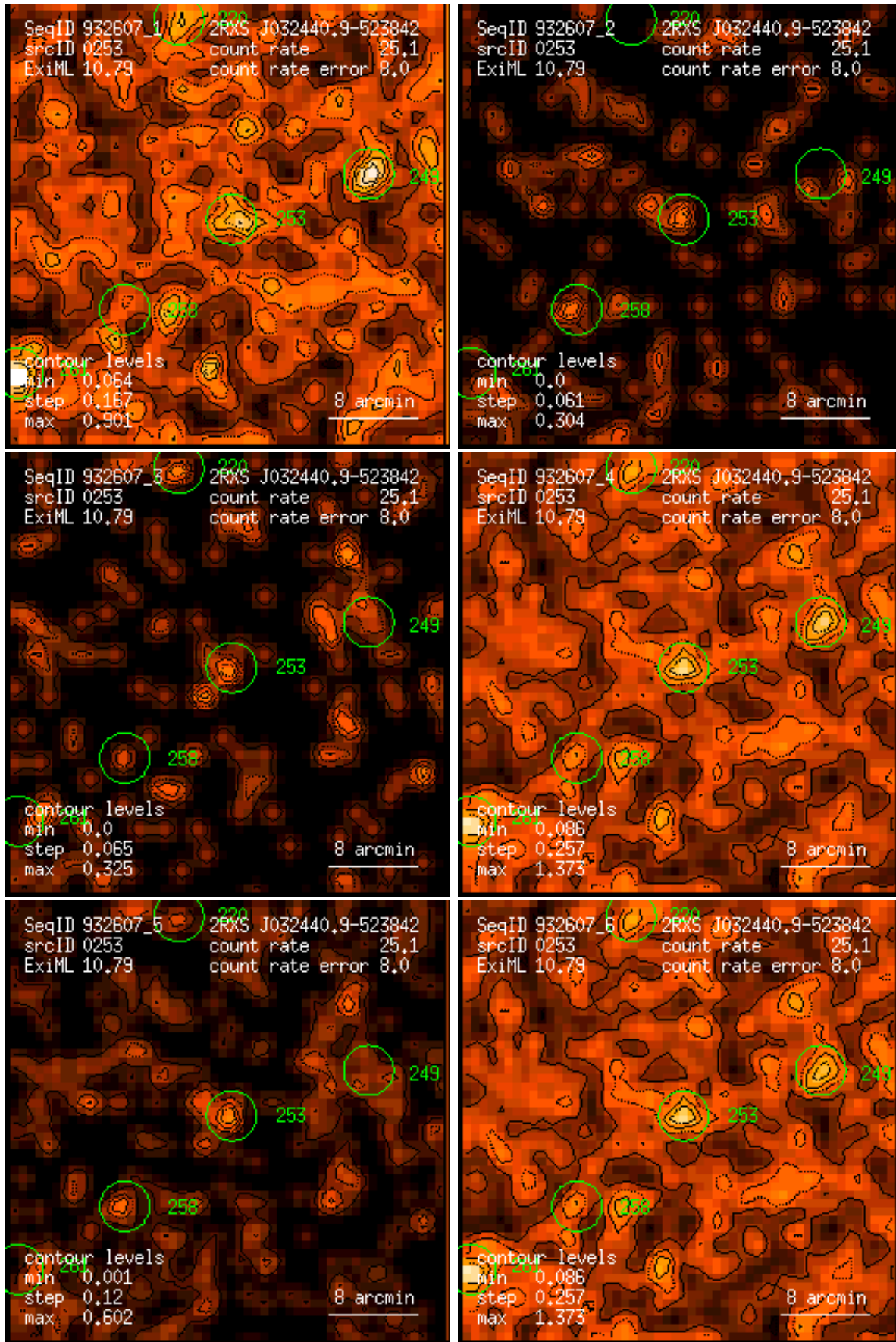
Figure 253: RASS 932607: detection 0253: band rate images, Gaussian filter: (1) PSPC channels 11 – 41, (2) 52 – 90, (3) 91 – 201, (4) 11 – 235, (5) 52 – 201, (6) 11 – 201. Broad band rates in counts/ks. Band rate contour levels in counts/ks/arcmin 2 .
