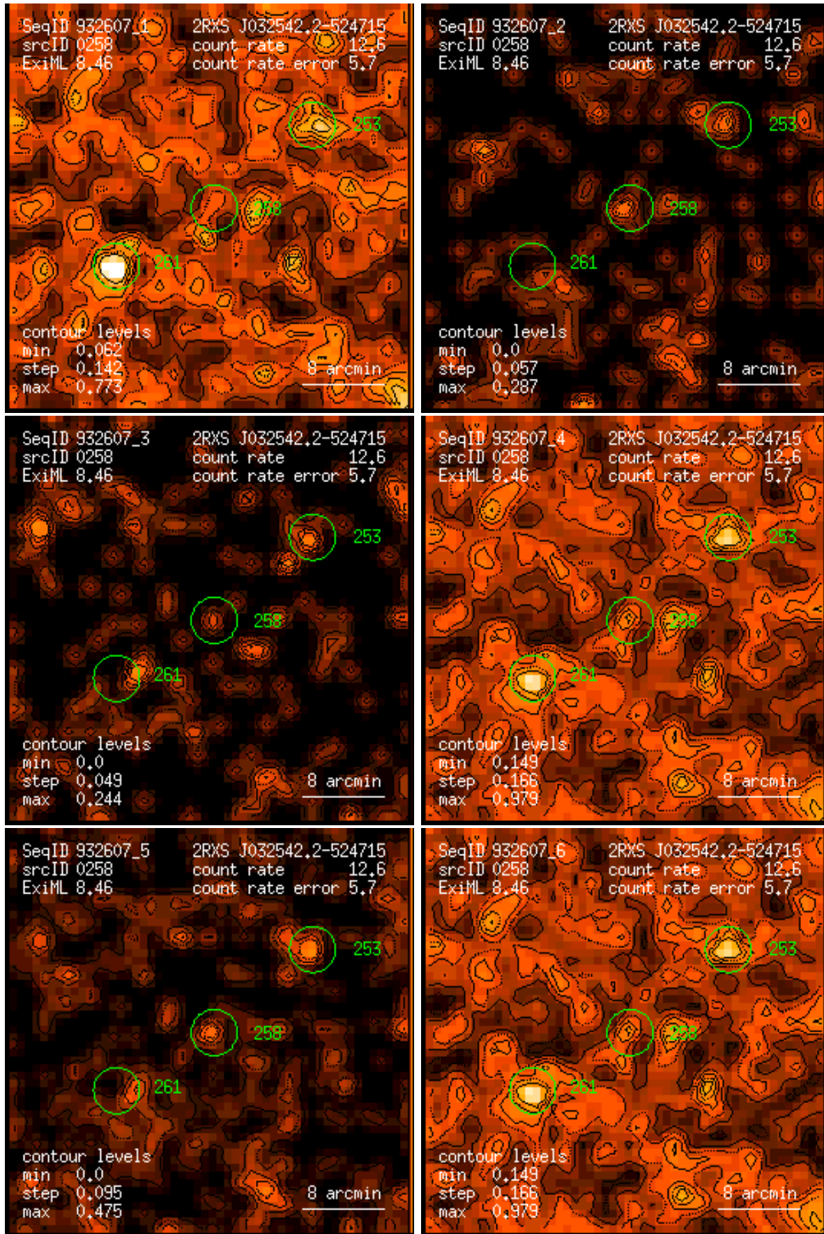
Figure 258: RASS 932607: detection 0258: band rate images, Gaussian filter: (1) PSPC channels 11 – 41, (2) 52 – 90, (3) 91 – 201, (4) 11 – 235, (5) 52 – 201, (6) 11 – 201. Broad band rates in counts/ks. Band rate contour levels in counts/ks/arcmin 2 .
