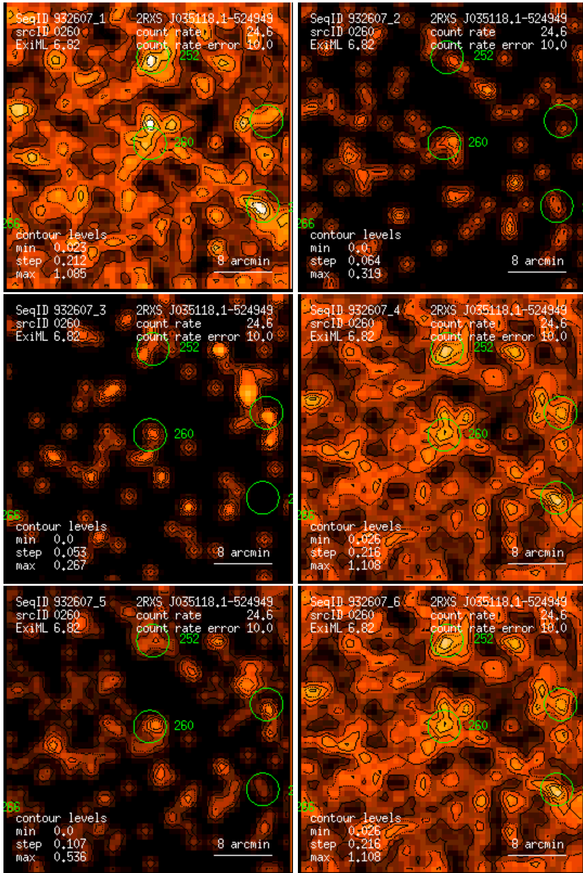
Figure 260: RASS 932607: detection 0260: band rate images, Gaussian filter: (1) PSPC channels 11 – 41, (2) 52 – 90, (3) 91 – 201, (4) 11 – 235, (5) 52 – 201, (6) 11 – 201. Broad band rates in counts/ks. Band rate contour levels in counts/ks/arcmin 2 .
