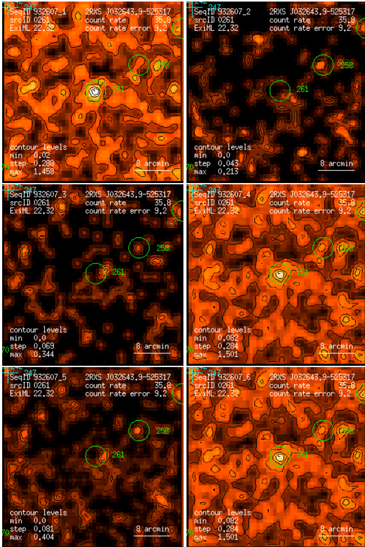
Figure 261: RASS 932607: detection 0261: band rate images, Gaussian filter: (1) PSPC channels 11 – 41, (2) 52 – 90, (3) 91 – 201, (4) 11 – 235, (5) 52 – 201, (6) 11 – 201. Broad band rates in counts/ks. Band rate contour levels in counts/ks/arcmin 2 .
