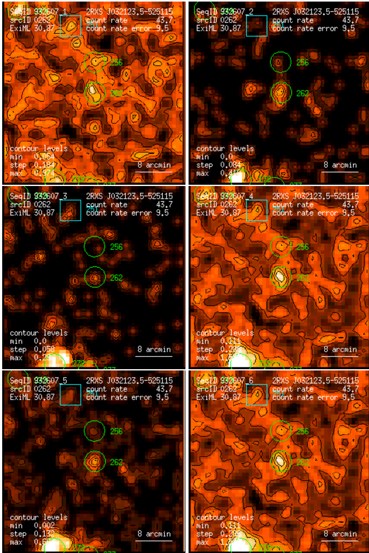
Figure 262: RASS 932607: detection 0262: band rate images, Gaussian filter: (1) PSPC channels 11 – 41, (2) 52 – 90, (3) 91 – 201, (4) 11 – 235, (5) 52 – 201, (6) 11 – 201. Broad band rates in counts/ks. Band rate contour levels in counts/ks/arcmin 2 .
