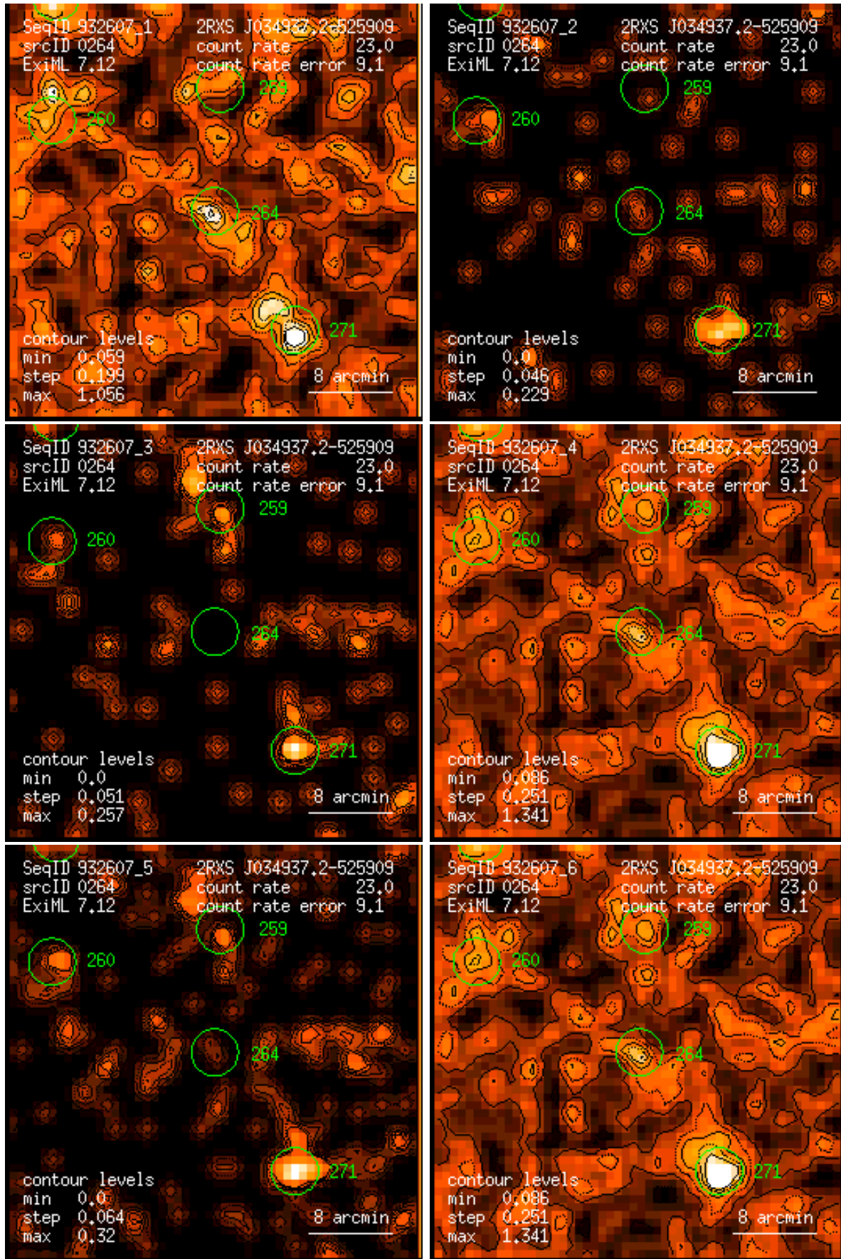
Figure 264: RASS 932607: detection 0264: band rate images, Gaussian filter: (1) PSPC channels 11 – 41, (2) 52 – 90, (3) 91 – 201, (4) 11 – 235, (5) 52 – 201, (6) 11 – 201. Broad band rates in counts/ks. Band rate contour levels in counts/ks/arcmin 2 .
