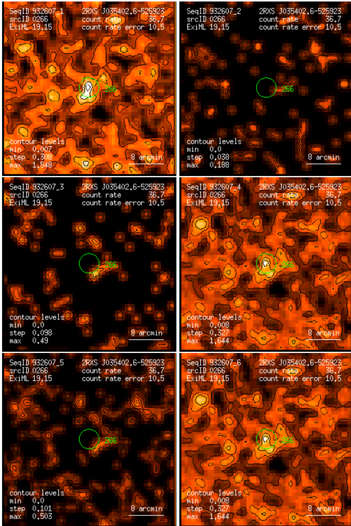
Figure 266: RASS 932607: detection 0266: band rate images, Gaussian filter: (1) PSPC channels 11 – 41, (2) 52 – 90, (3) 91 – 201, (4) 11 – 235, (5) 52 – 201, (6) 11 – 201. Broad band rates in counts/ks. Band rate contour levels in counts/ks/arcmin 2 .
