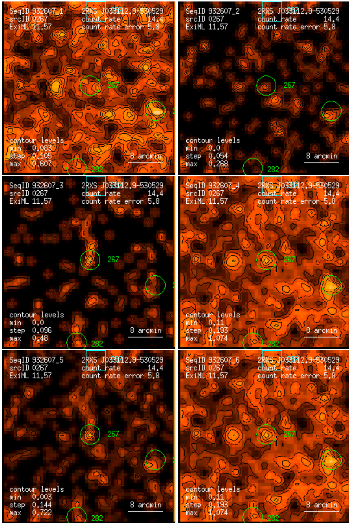
Figure 267: RASS 932607: detection 0267: band rate images, Gaussian filter: (1) PSPC channels 11 – 41, (2) 52 – 90, (3) 91 – 201, (4) 11 – 235, (5) 52 – 201, (6) 11 – 201. Broad band rates in counts/ks. Band rate contour levels in counts/ks/arcmin 2 .
