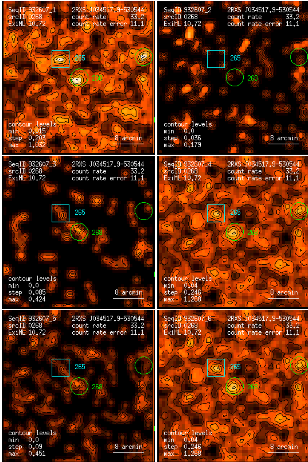
Figure 268: RASS 932607: detection 0268: band rate images, Gaussian filter: (1) PSPC channels 11 – 41, (2) 52 – 90, (3) 91 – 201, (4) 11 – 235, (5) 52 – 201, (6) 11 – 201. Broad band rates in counts/ks. Band rate contour levels in counts/ks/arcmin 2 .
