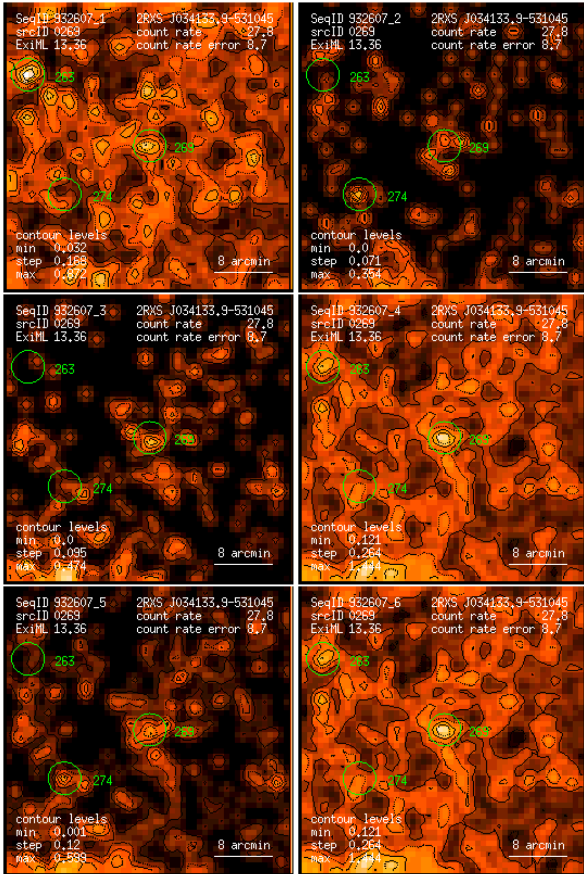
Figure 269: RASS 932607: detection 0269: band rate images, Gaussian filter: (1) PSPC channels 11 – 41, (2) 52 – 90, (3) 91 – 201, (4) 11 – 235, (5) 52 – 201, (6) 11 – 201. Broad band rates in counts/ks. Band rate contour levels in counts/ks/arcmin 2 .
