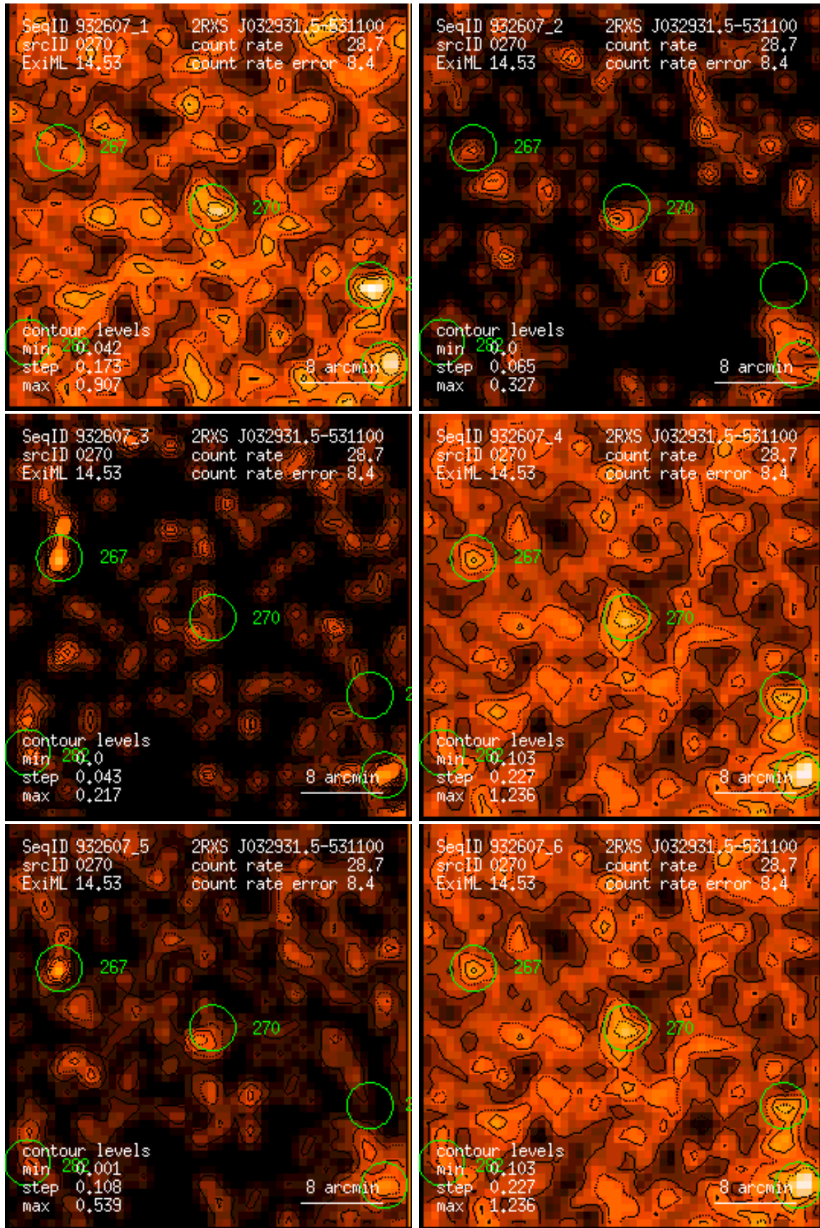
Figure 270: RASS 932607: detection 0270: band rate images, Gaussian filter: (1) PSPC channels 11 – 41, (2) 52 – 90, (3) 91 – 201, (4) 11 – 235, (5) 52 – 201, (6) 11 – 201. Broad band rates in counts/ks. Band rate contour levels in counts/ks/arcmin 2 .
