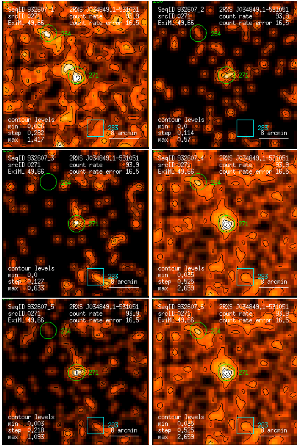
Figure 271: RASS 932607: detection 0271: band rate images, Gaussian filter: (1) PSPC channels 11 – 41, (2) 52 – 90, (3) 91 – 201, (4) 11 – 235, (5) 52 – 201, (6) 11 – 201. Broad band rates in counts/ks. Band rate contour levels in counts/ks/arcmin 2 .
