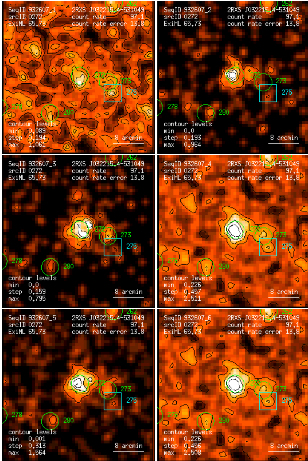
Figure 272: RASS 932607: detection 0272: band rate images, Gaussian filter: (1) PSPC channels 11 – 41, (2) 52 – 90, (3) 91 – 201, (4) 11 – 235, (5) 52 – 201, (6) 11 – 201. Broad band rates in counts/ks. Band rate contour levels in counts/ks/arcmin 2 .
