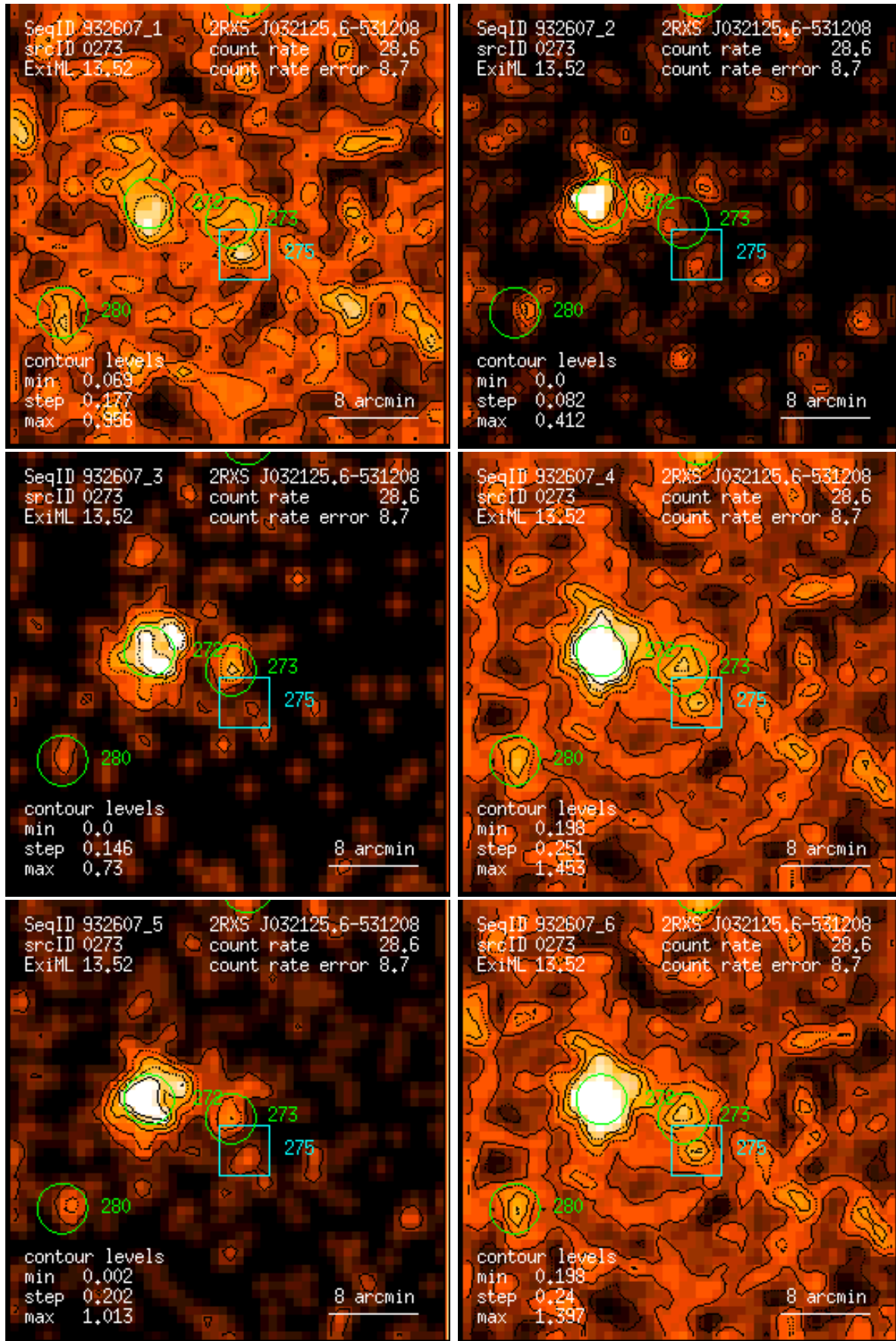
Figure 273: RASS 932607: detection 0273: band rate images, Gaussian filter: (1) PSPC channels 11 – 41, (2) 52 – 90, (3) 91 – 201, (4) 11 – 235, (5) 52 – 201, (6) 11 – 201. Broad band rates in counts/ks. Band rate contour levels in counts/ks/arcmin 2 .
