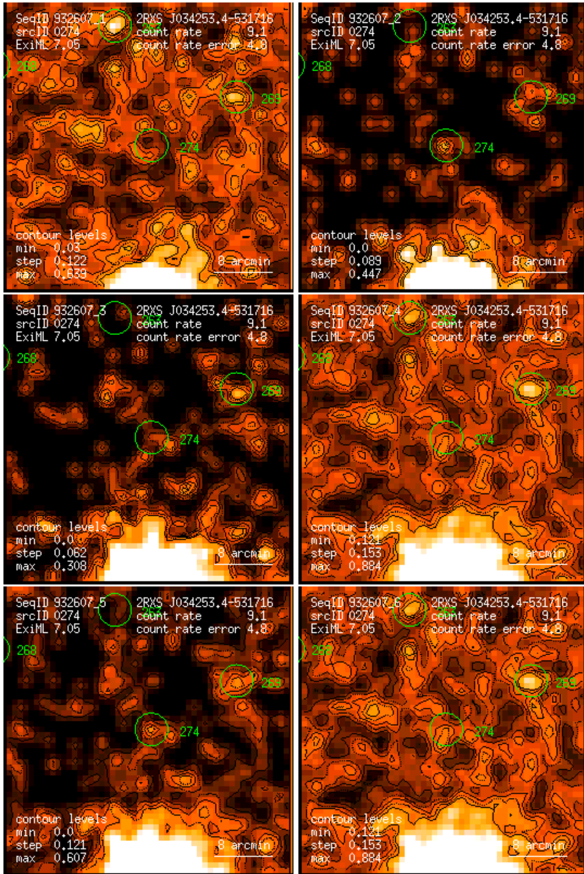
Figure 274: RASS 932607: detection 0274: band rate images, Gaussian filter: (1) PSPC channels 11 – 41, (2) 52 – 90, (3) 91 – 201, (4) 11 – 235, (5) 52 – 201, (6) 11 – 201. Broad band rates in counts/ks. Band rate contour levels in counts/ks/arcmin 2 .
