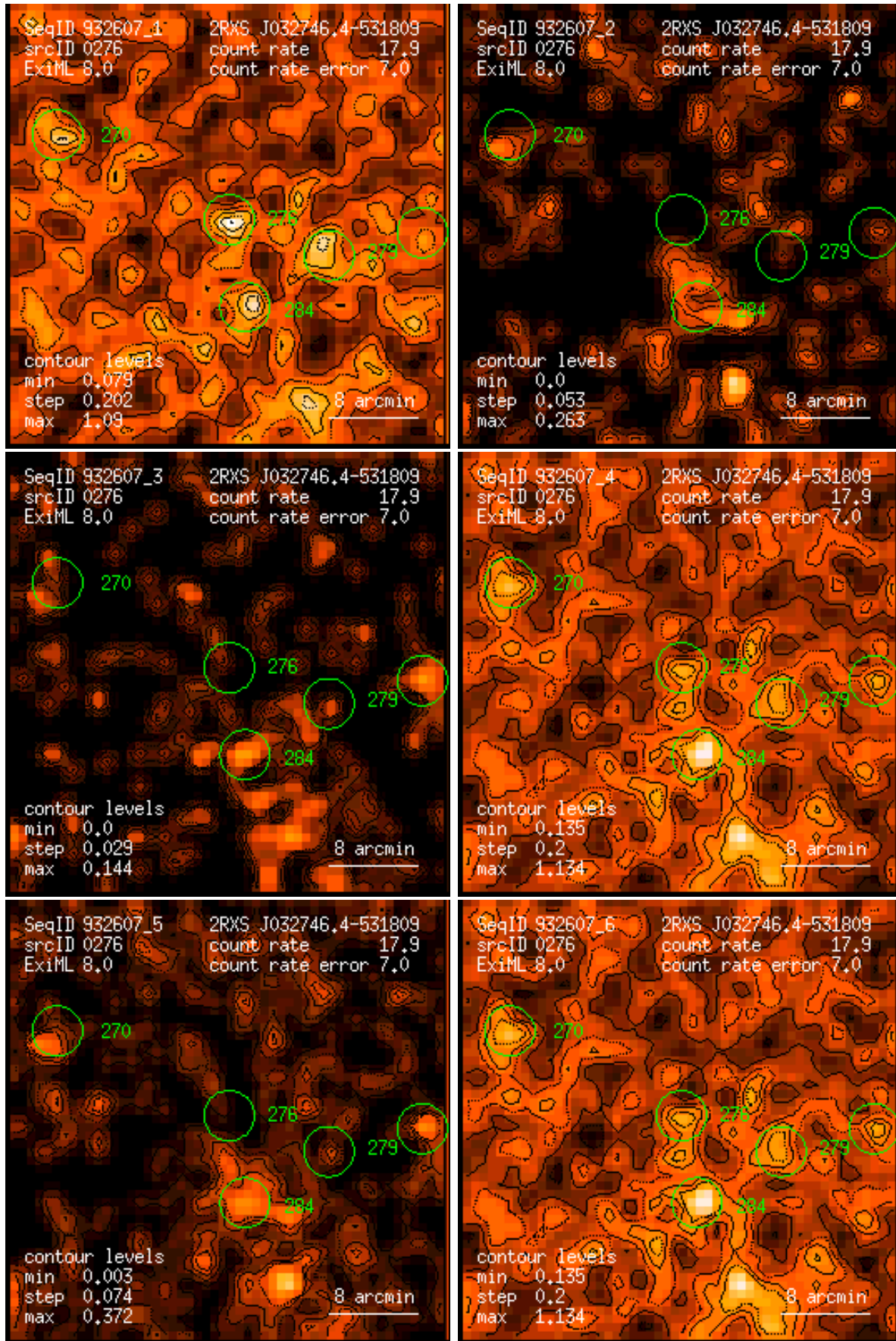
Figure 276: RASS 932607: detection 0276: band rate images, Gaussian filter: (1) PSPC channels 11 – 41, (2) 52 – 90, (3) 91 – 201, (4) 11 – 235, (5) 52 – 201, (6) 11 – 201. Broad band rates in counts/ks. Band rate contour levels in counts/ks/arcmin 2 .
