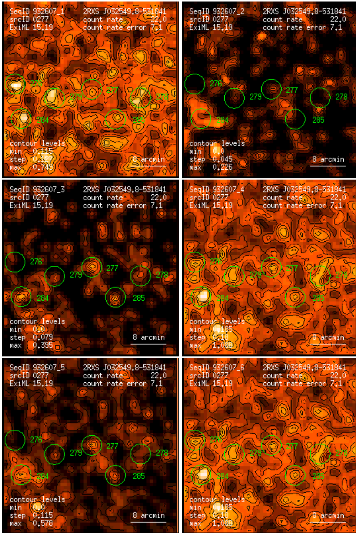
Figure 277: RASS 932607: detection 0277: band rate images, Gaussian filter: (1) PSPC channels 11 – 41, (2) 52 – 90, (3) 91 – 201, (4) 11 – 235, (5) 52 – 201, (6) 11 – 201. Broad band rates in counts/ks. Band rate contour levels in counts/ks/arcmin 2 .
