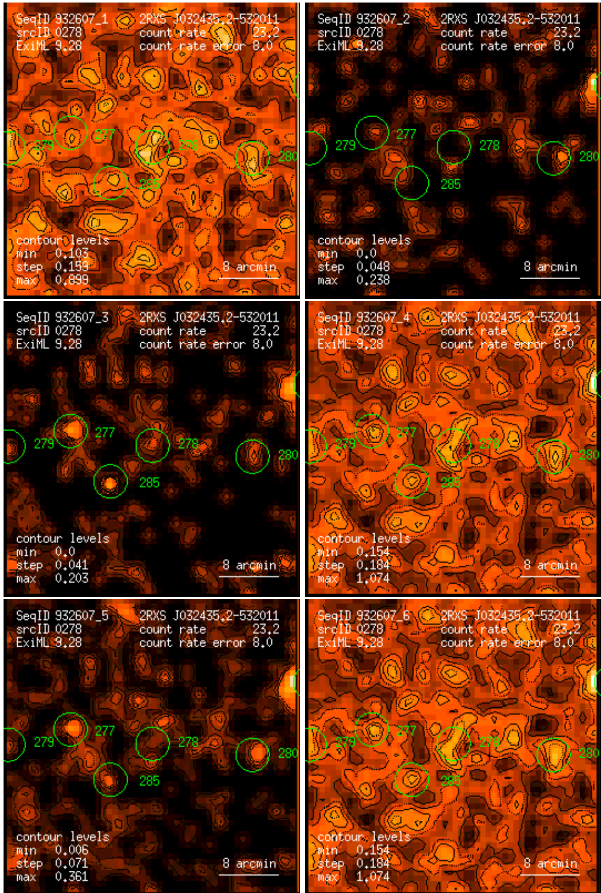
Figure 278: RASS 932607: detection 0278: band rate images, Gaussian filter: (1) PSPC channels 11 – 41, (2) 52 – 90, (3) 91 – 201, (4) 11 – 235, (5) 52 – 201, (6) 11 – 201. Broad band rates in counts/ks. Band rate contour levels in counts/ks/arcmin 2 .
