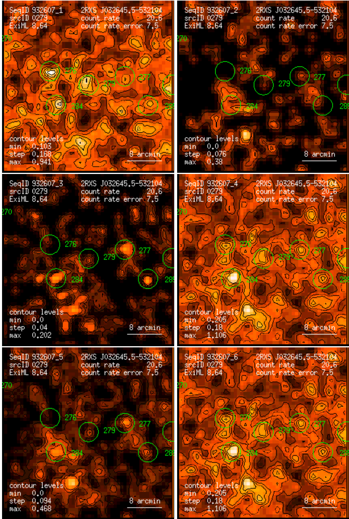
Figure 279: RASS 932607: detection 0279: band rate images, Gaussian filter: (1) PSPC channels 11 – 41, (2) 52 – 90, (3) 91 – 201, (4) 11 – 235, (5) 52 – 201, (6) 11 – 201. Broad band rates in counts/ks. Band rate contour levels in counts/ks/arcmin 2 .
