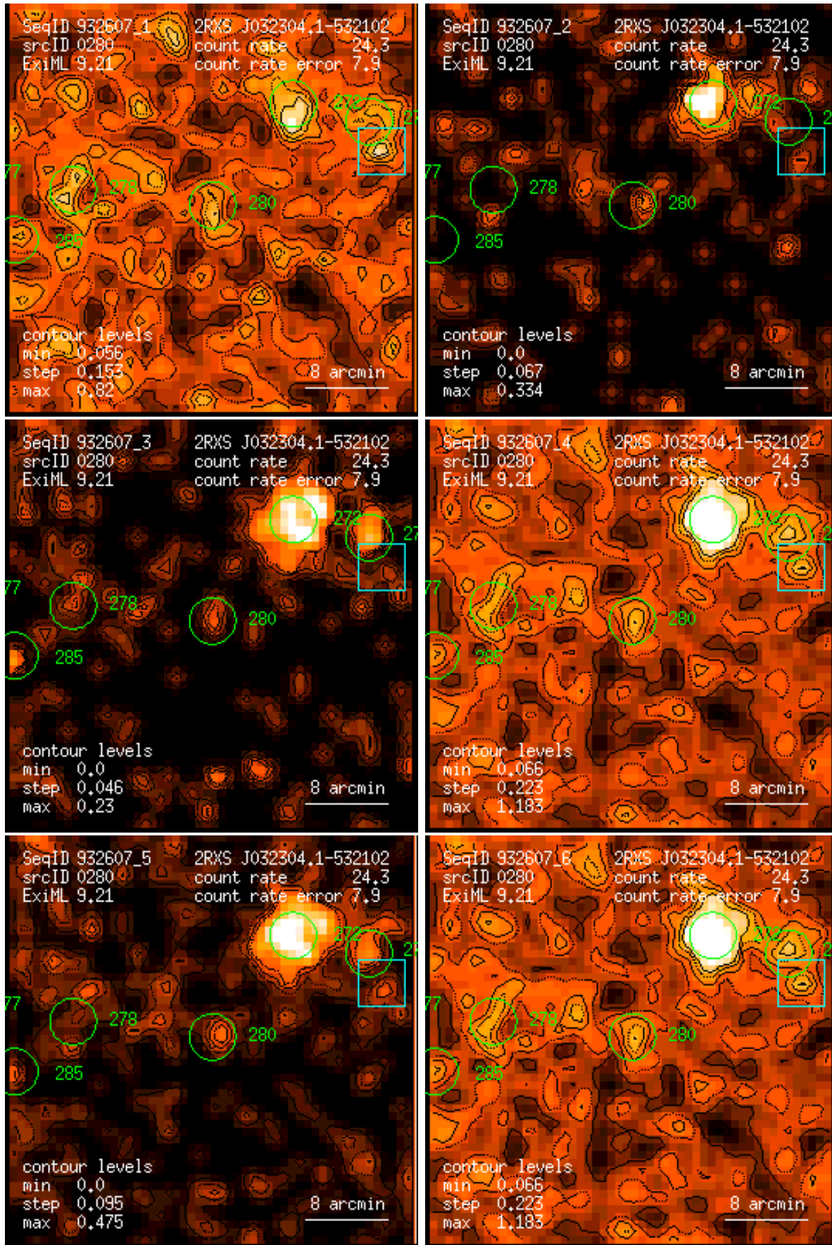
Figure 280: RASS 932607: detection 0280: band rate images, Gaussian filter: (1) PSPC channels 11 – 41, (2) 52 – 90, (3) 91 – 201, (4) 11 – 235, (5) 52 – 201, (6) 11 – 201. Broad band rates in counts/ks. Band rate contour levels in counts/ks/arcmin 2 .
