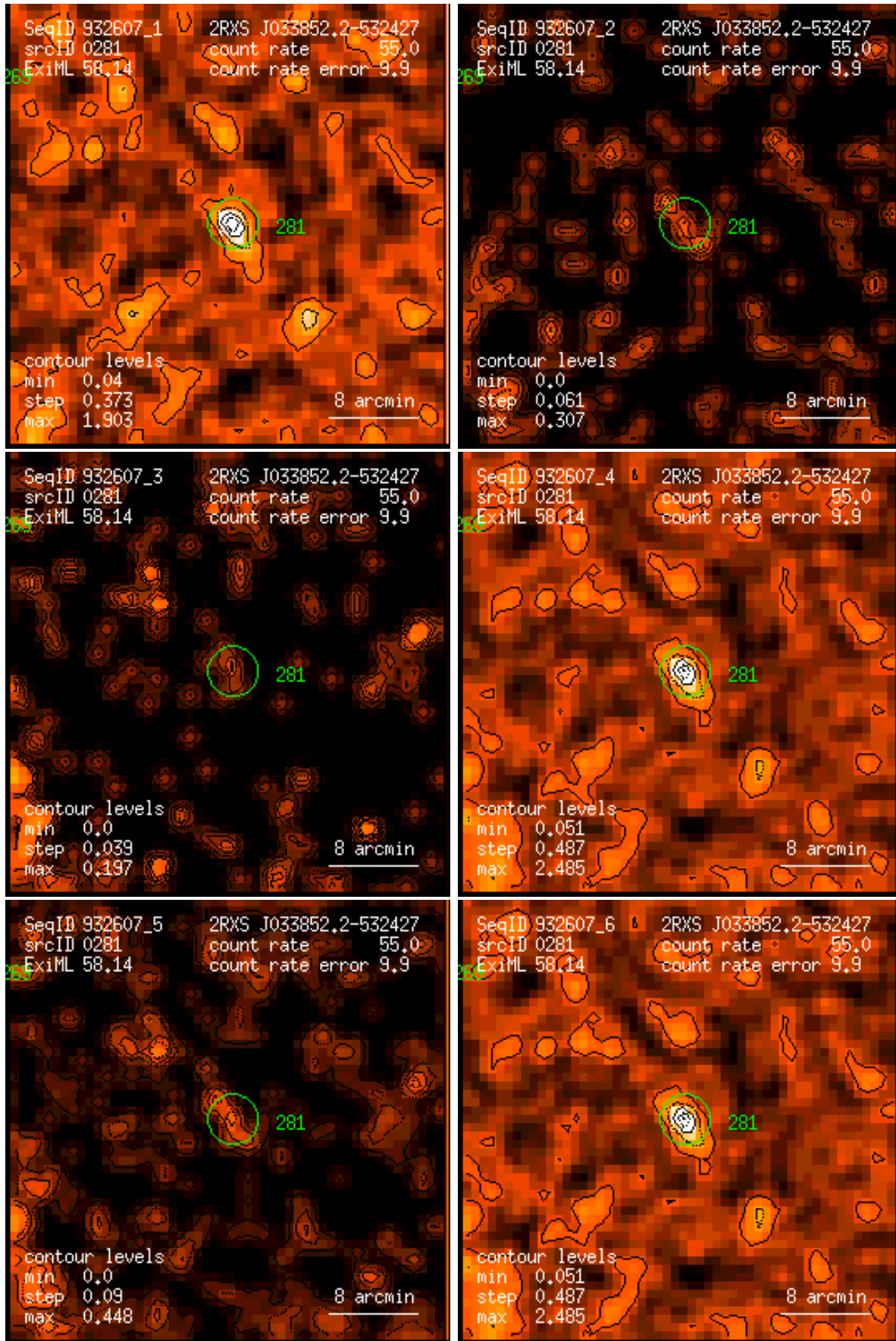
Figure 281: RASS 932607: detection 0281: band rate images, Gaussian filter: (1) PSPC channels 11 – 41, (2) 52 – 90, (3) 91 – 201, (4) 11 – 235, (5) 52 – 201, (6) 11 – 201. Broad band rates in counts/ks. Band rate contour levels in counts/ks/arcmin 2 .
