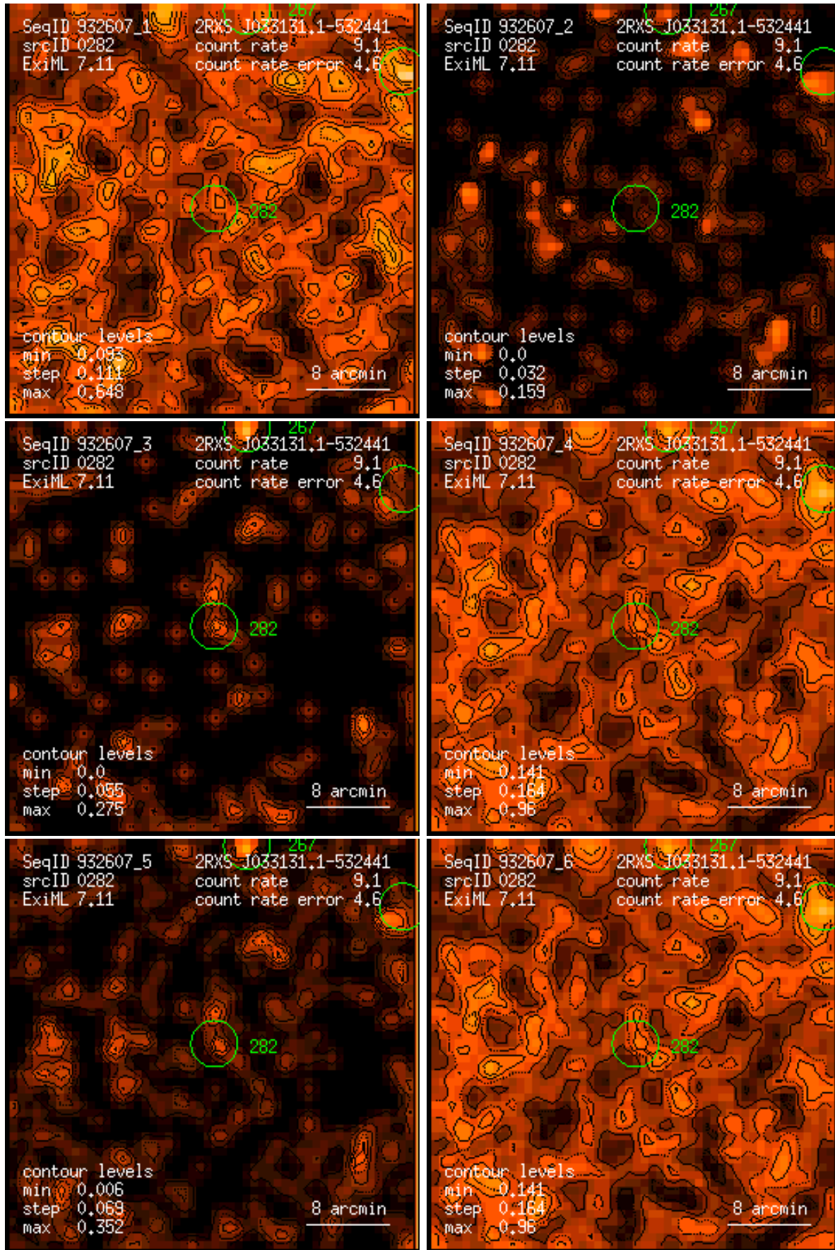
Figure 282: RASS 932607: detection 0282: band rate images, Gaussian filter: (1) PSPC channels 11 – 41, (2) 52 – 90, (3) 91 – 201, (4) 11 – 235, (5) 52 – 201, (6) 11 – 201. Broad band rates in counts/ks. Band rate contour levels in counts/ks/arcmin 2 .
