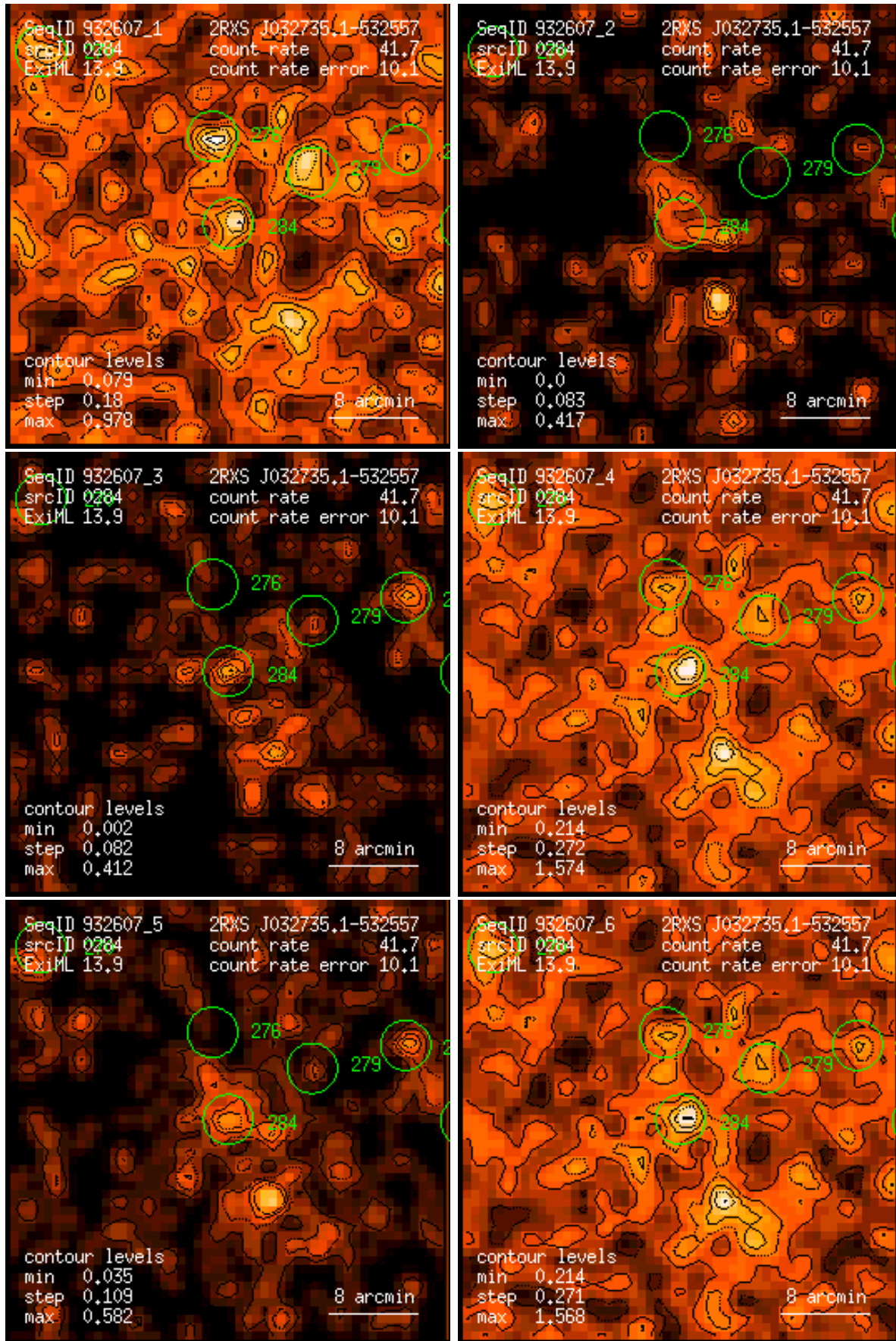
Figure 284: RASS 932607: detection 0284: band rate images, Gaussian filter: (1) PSPC channels 11 – 41, (2) 52 – 90, (3) 91 – 201, (4) 11 – 235, (5) 52 – 201, (6) 11 – 201. Broad band rates in counts/ks. Band rate contour levels in counts/ks/arcmin 2 .
