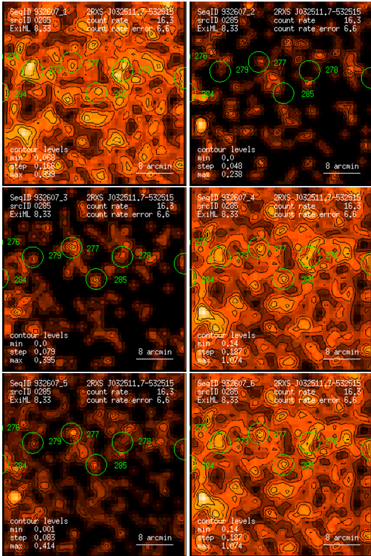
Figure 285: RASS 932607: detection 0285: band rate images, Gaussian filter: (1) PSPC channels 11 – 41, (2) 52 – 90, (3) 91 – 201, (4) 11 – 235, (5) 52 – 201, (6) 11 – 201. Broad band rates in counts/ks. Band rate contour levels in counts/ks/arcmin 2 .
