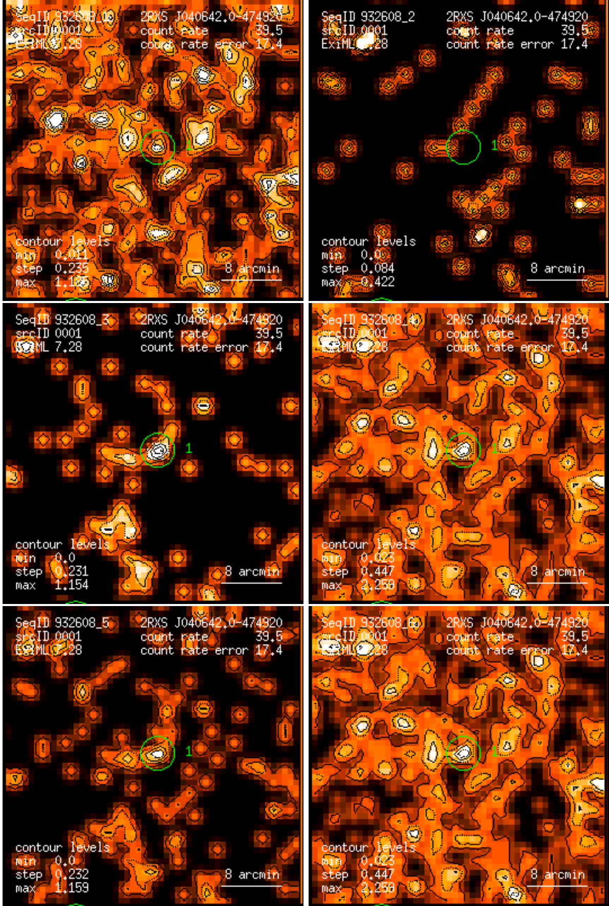
Figure 1: RASS 932608: detection 0001: band rate images, Gaussian filter: (1) PSPC channels 11 – 41, (2) 52 – 90, (3) 91 – 201, (4) 11 – 235, (5) 52 – 201, (6) 11 – 201. Broad band rates in counts/ks. Band rate contour levels in counts/ks/arcmin 2 .
